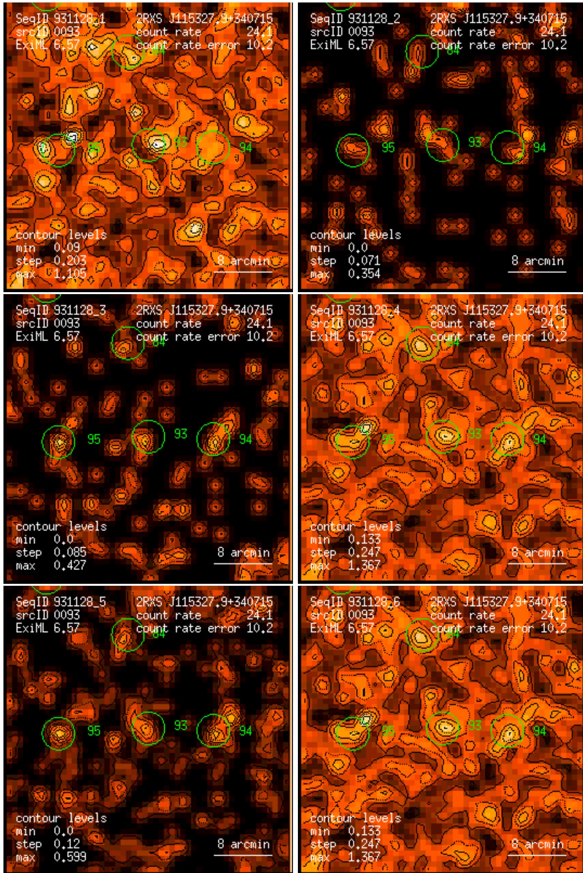
Figure 93: RASS 931128: detection 0093: band rate images, Gaussian filter: (1) PSPC channels 11 – 41, (2) 52 – 90, (3) 91 – 201, (4) 11 – 235, (5) 52 – 201, (6) 11 – 201. Broad band rates in counts/ks. Band rate contour levels in counts/ks/arcmin 2 .
