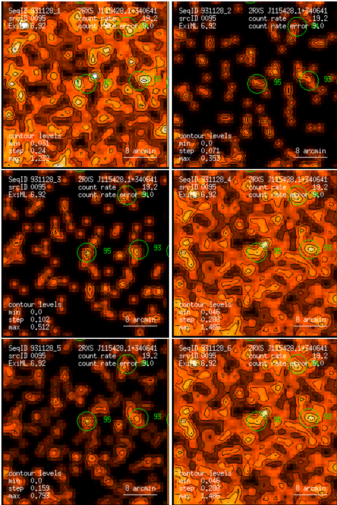
Figure 95: RASS 931128: detection 0095: band rate images, Gaussian filter: (1) PSPC channels 11 – 41, (2) 52 – 90, (3) 91 – 201, (4) 11 – 235, (5) 52 – 201, (6) 11 – 201. Broad band rates in counts/ks. Band rate contour levels in counts/ks/arcmin 2 .
