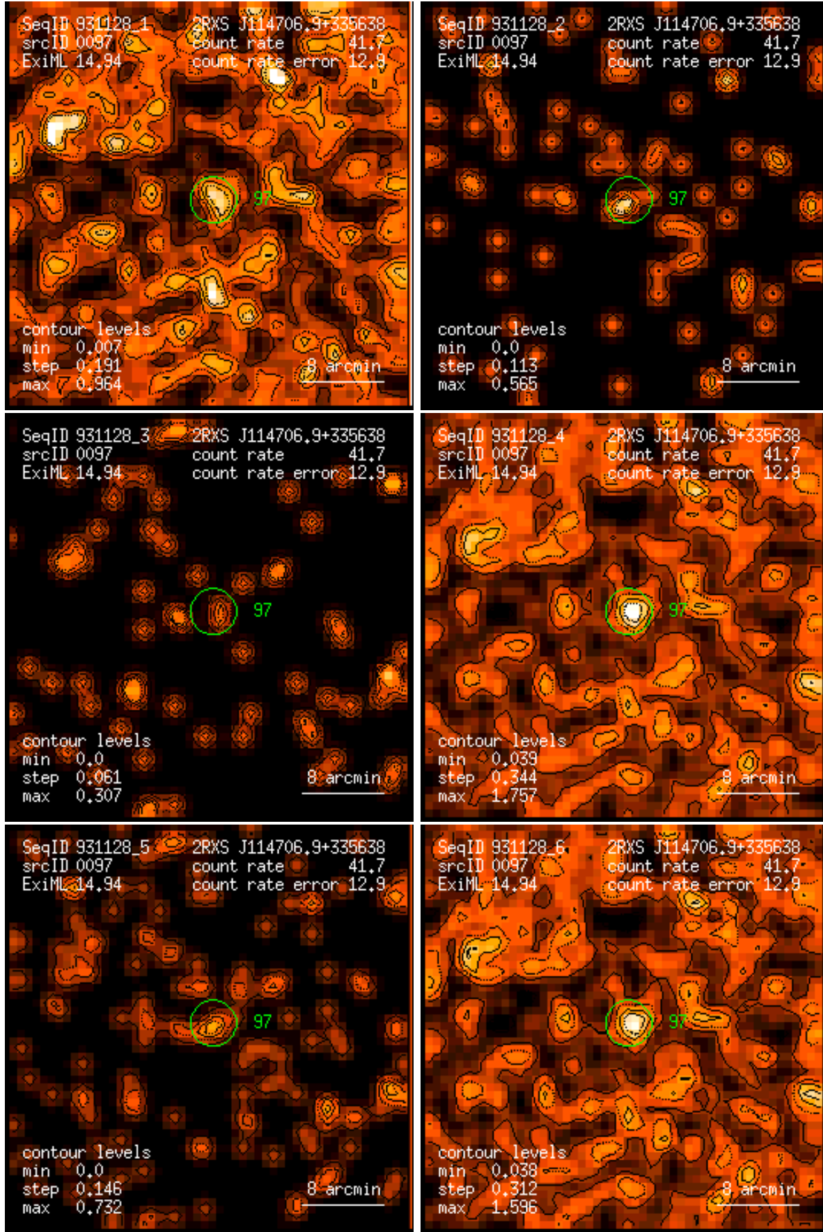
Figure 97: RASS 931128: detection 0097: band rate images, Gaussian filter: (1) PSPC channels 11 – 41, (2) 52 – 90, (3) 91 – 201, (4) 11 – 235, (5) 52 – 201, (6) 11 – 201. Broad band rates in counts/ks. Band rate contour levels in counts/ks/arcmin 2 .
