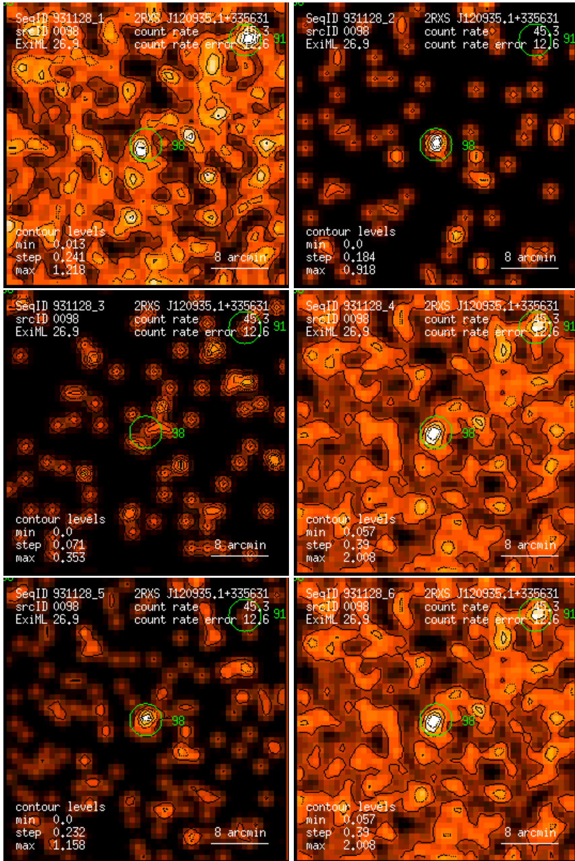
Figure 98: RASS 931128: detection 0098: band rate images, Gaussian filter: (1) PSPC channels 11 – 41, (2) 52 – 90, (3) 91 – 201, (4) 11 – 235, (5) 52 – 201, (6) 11 – 201. Broad band rates in counts/ks. Band rate contour levels in counts/ks/arcmin 2 .
