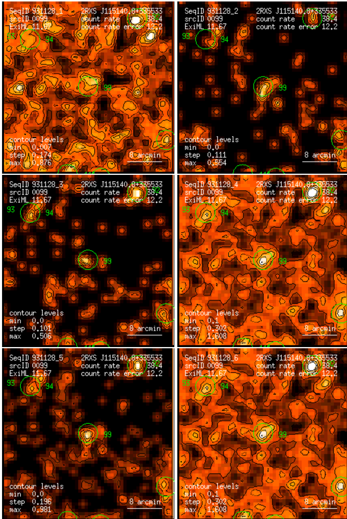
Figure 99: RASS 931128: detection 0099: band rate images, Gaussian filter: (1) PSPC channels 11 – 41, (2) 52 – 90, (3) 91 – 201, (4) 11 – 235, (5) 52 – 201, (6) 11 – 201. Broad band rates in counts/ks. Band rate contour levels in counts/ks/arcmin 2 .
