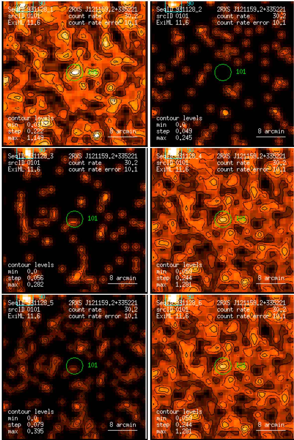
Figure 101: RASS 931128: detection 0101: band rate images, Gaussian filter: (1) PSPC channels 11 – 41, (2) 52 – 90, (3) 91 – 201, (4) 11 – 235, (5) 52 – 201, (6) 11 – 201. Broad band rates in counts/ks. Band rate contour levels in counts/ks/arcmin 2 .
