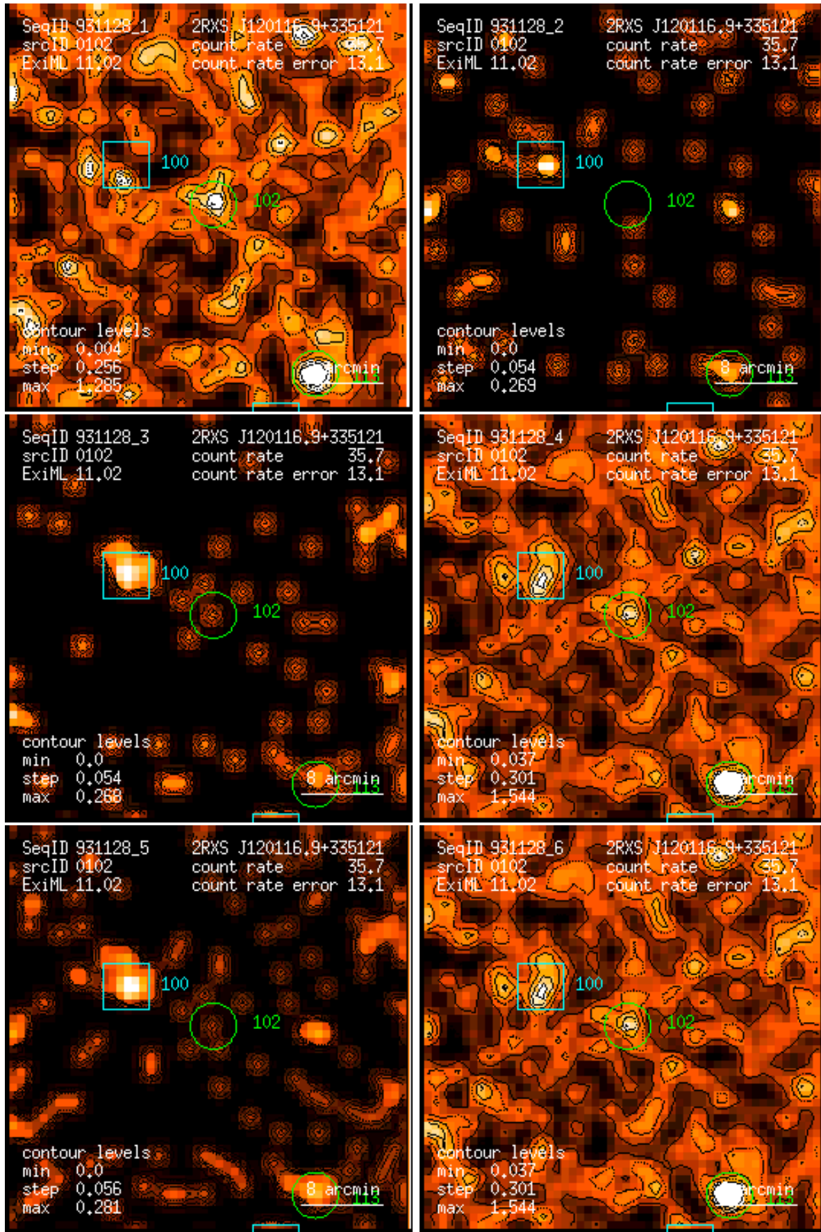
Figure 102: RASS 931128: detection 0102: band rate images, Gaussian filter: (1) PSPC channels 11 – 41, (2) 52 – 90, (3) 91 – 201, (4) 11 – 235, (5) 52 – 201, (6) 11 – 201. Broad band rates in counts/ks. Band rate contour levels in counts/ks/arcmin 2 .
