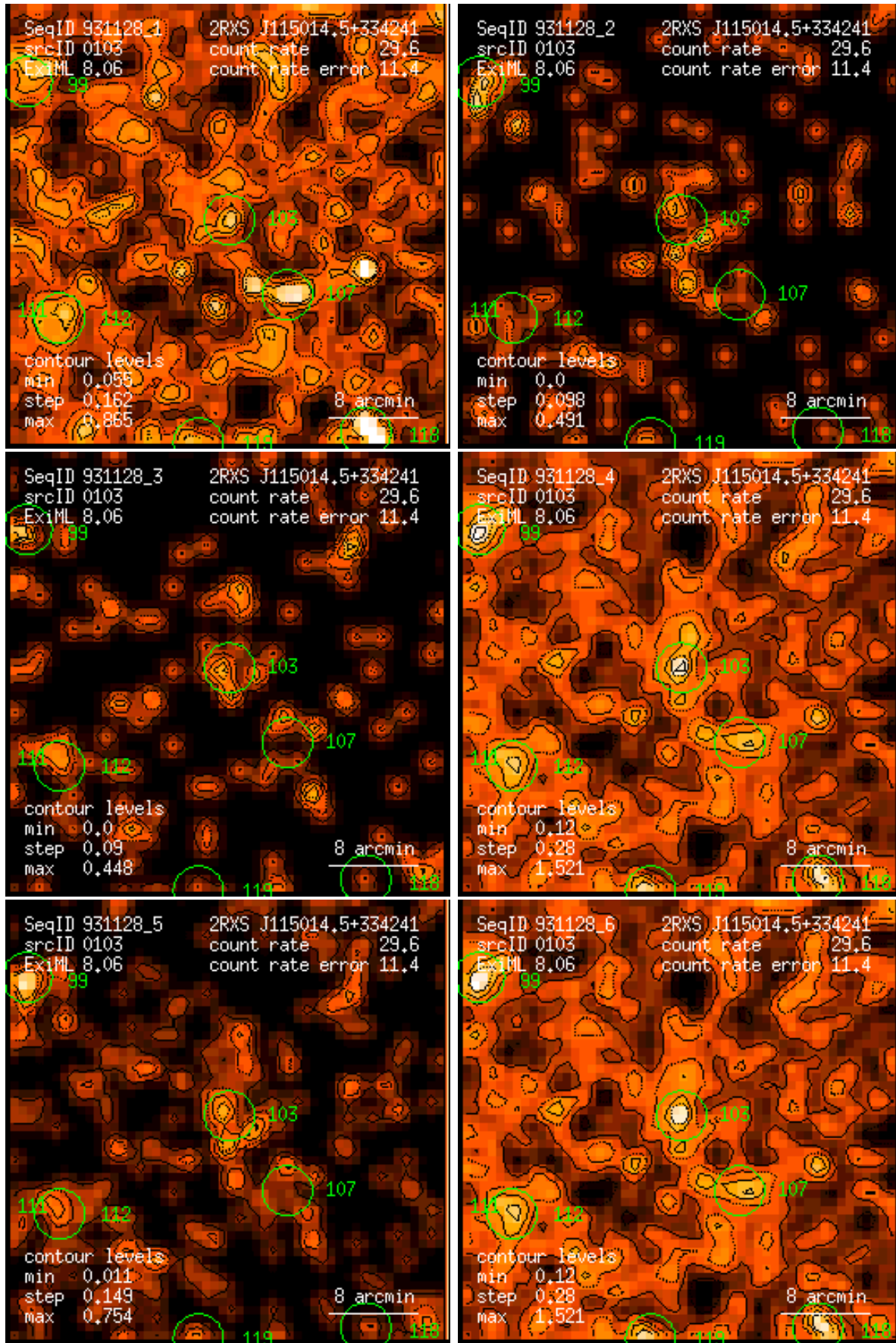
Figure 103: RASS 931128: detection 0103: band rate images, Gaussian filter: (1) PSPC channels 11 – 41, (2) 52 – 90, (3) 91 – 201, (4) 11 – 235, (5) 52 – 201, (6) 11 – 201. Broad band rates in counts/ks. Band rate contour levels in counts/ks/arcmin 2 .
