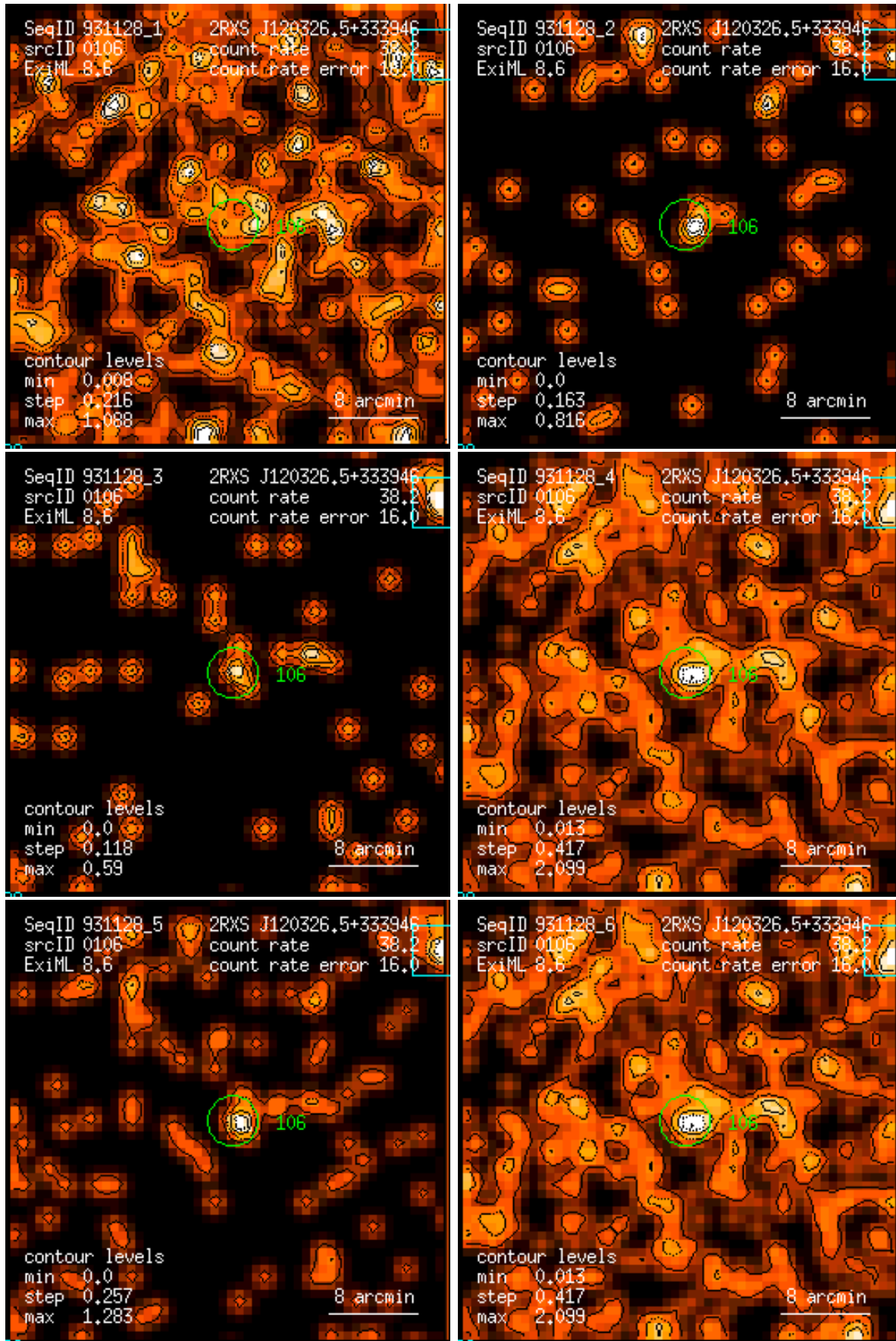
Figure 106: RASS 931128: detection 0106: band rate images, Gaussian filter: (1) PSPC channels 11 – 41, (2) 52 – 90, (3) 91 – 201, (4) 11 – 235, (5) 52 – 201, (6) 11 – 201. Broad band rates in counts/ks. Band rate contour levels in counts/ks/arcmin 2 .
