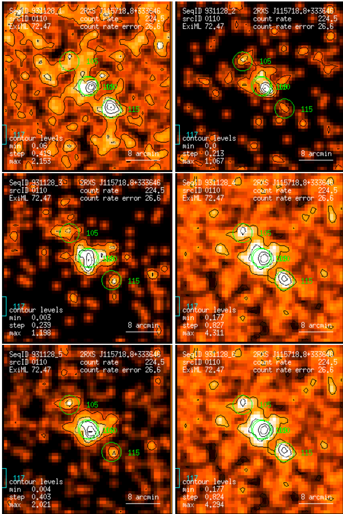
Figure 110: RASS 931128: detection 0110: band rate images, Gaussian filter: (1) PSPC channels 11 – 41, (2) 52 – 90, (3) 91 – 201, (4) 11 – 235, (5) 52 – 201, (6) 11 – 201. Broad band rates in counts/ks. Band rate contour levels in counts/ks/arcmin 2 .
