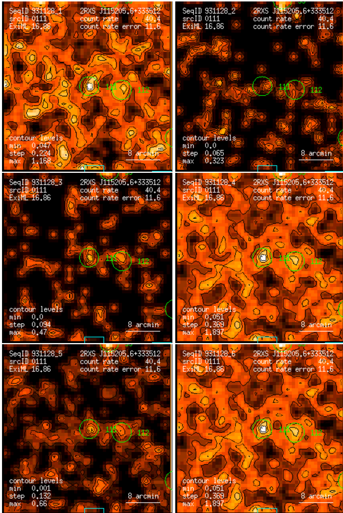
Figure 111: RASS 931128: detection 0111: band rate images, Gaussian filter: (1) PSPC channels 11 – 41, (2) 52 – 90, (3) 91 – 201, (4) 11 – 235, (5) 52 – 201, (6) 11 – 201. Broad band rates in counts/ks. Band rate contour levels in counts/ks/arcmin 2 .
