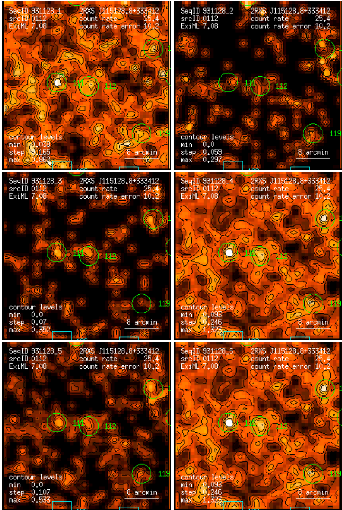
Figure 112: RASS 931128: detection 0112: band rate images, Gaussian filter: (1) PSPC channels 11 – 41, (2) 52 – 90, (3) 91 – 201, (4) 11 – 235, (5) 52 – 201, (6) 11 – 201. Broad band rates in counts/ks. Band rate contour levels in counts/ks/arcmin 2 .
