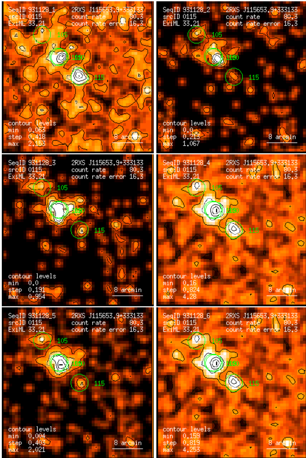
Figure 115: RASS 931128: detection 0115: band rate images, Gaussian filter: (1) PSPC channels 11 – 41, (2) 52 – 90, (3) 91 – 201, (4) 11 – 235, (5) 52 – 201, (6) 11 – 201. Broad band rates in counts/ks. Band rate contour levels in counts/ks/arcmin 2 .
