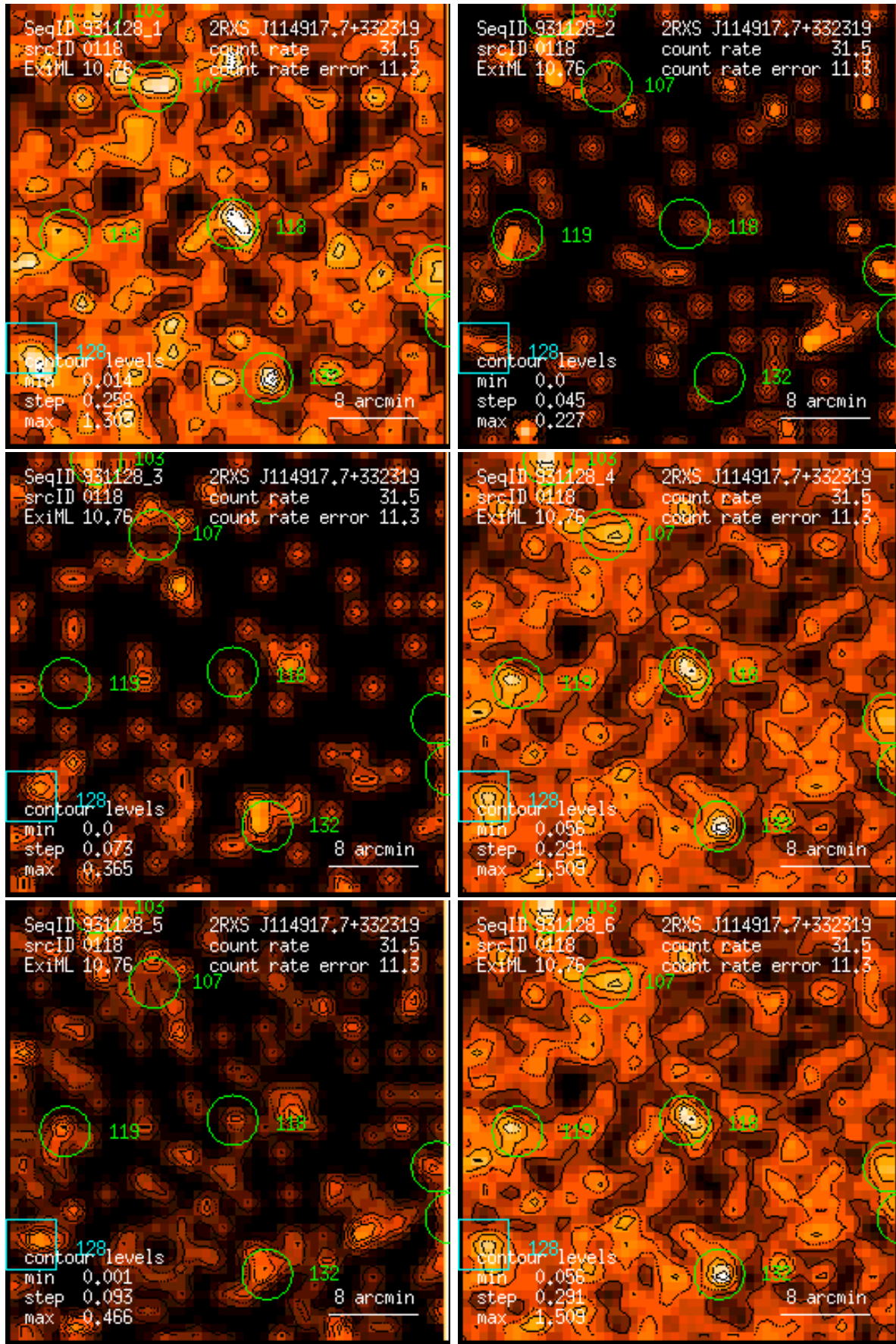
Figure 118: RASS 931128: detection 0118: band rate images, Gaussian filter: (1) PSPC channels 11 – 41, (2) 52 – 90, (3) 91 – 201, (4) 11 – 235, (5) 52 – 201, (6) 11 – 201. Broad band rates in counts/ks. Band rate contour levels in counts/ks/arcmin 2 .
