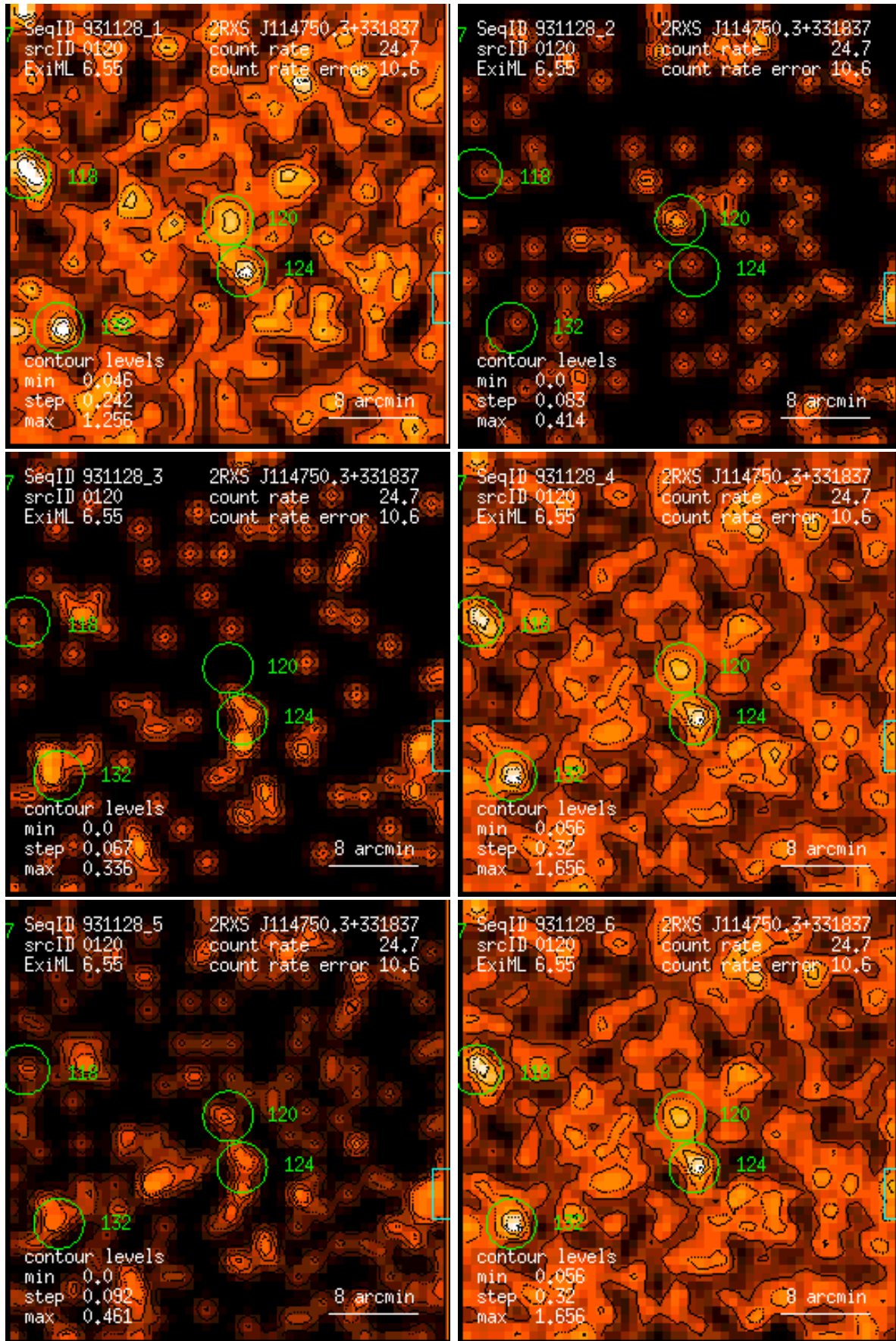
Figure 120: RASS 931128: detection 0120: band rate images, Gaussian filter: (1) PSPC channels 11 – 41, (2) 52 – 90, (3) 91 – 201, (4) 11 – 235, (5) 52 – 201, (6) 11 – 201. Broad band rates in counts/ks. Band rate contour levels in counts/ks/arcmin 2 .
