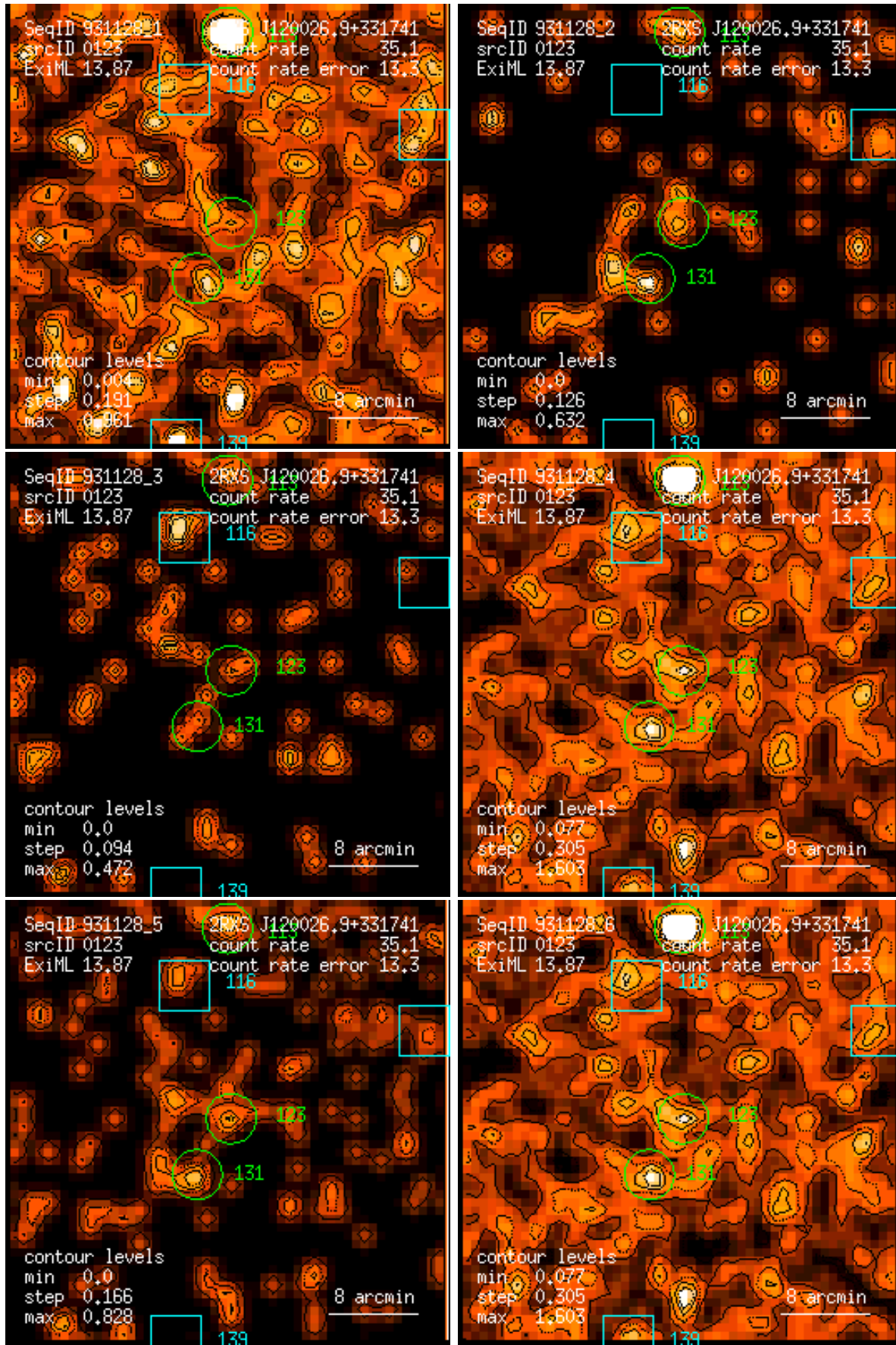
Figure 123: RASS 931128: detection 0123: band rate images, Gaussian filter: (1) PSPC channels 11 – 41, (2) 52 – 90, (3) 91 – 201, (4) 11 – 235, (5) 52 – 201, (6) 11 – 201. Broad band rates in counts/ks. Band rate contour levels in counts/ks/arcmin 2 .
