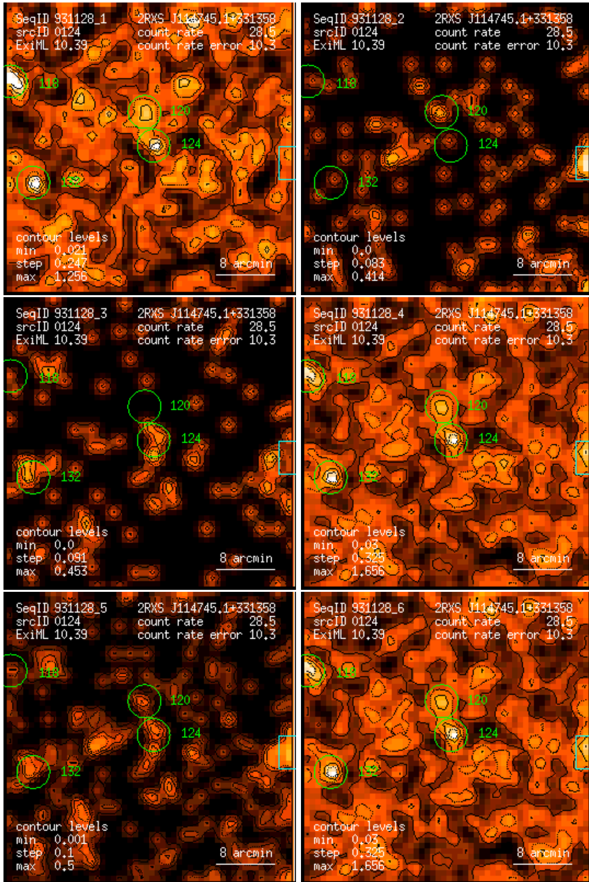
Figure 124: RASS 931128: detection 0124: band rate images, Gaussian filter: (1) PSPC channels 11 – 41, (2) 52 – 90, (3) 91 – 201, (4) 11 – 235, (5) 52 – 201, (6) 11 – 201. Broad band rates in counts/ks. Band rate contour levels in counts/ks/arcmin 2 .
