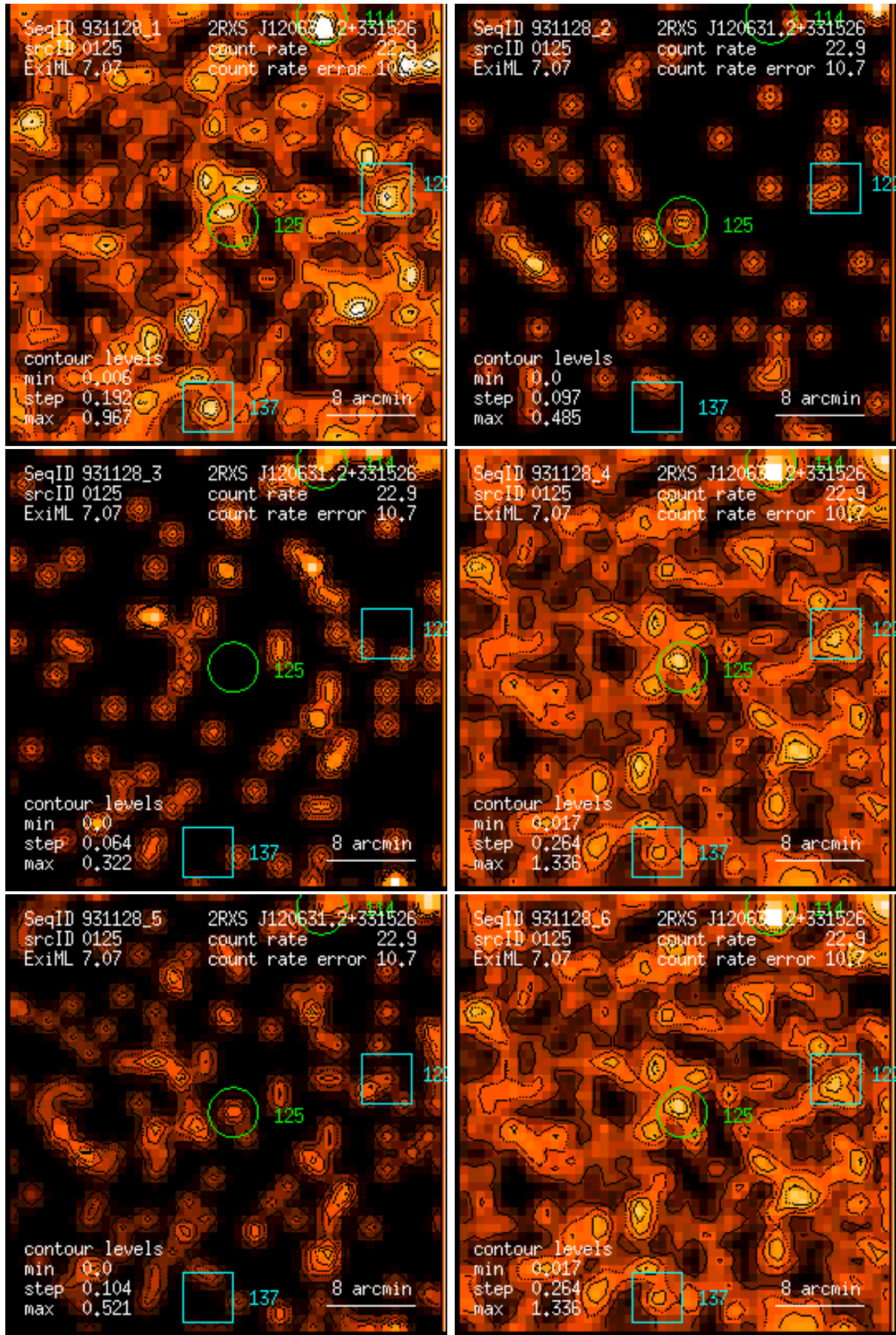
Figure 125: RASS 931128: detection 0125: band rate images, Gaussian filter: (1) PSPC channels 11 – 41, (2) 52 – 90, (3) 91 – 201, (4) 11 – 235, (5) 52 – 201, (6) 11 – 201. Broad band rates in counts/ks. Band rate contour levels in counts/ks/arcmin 2 .
