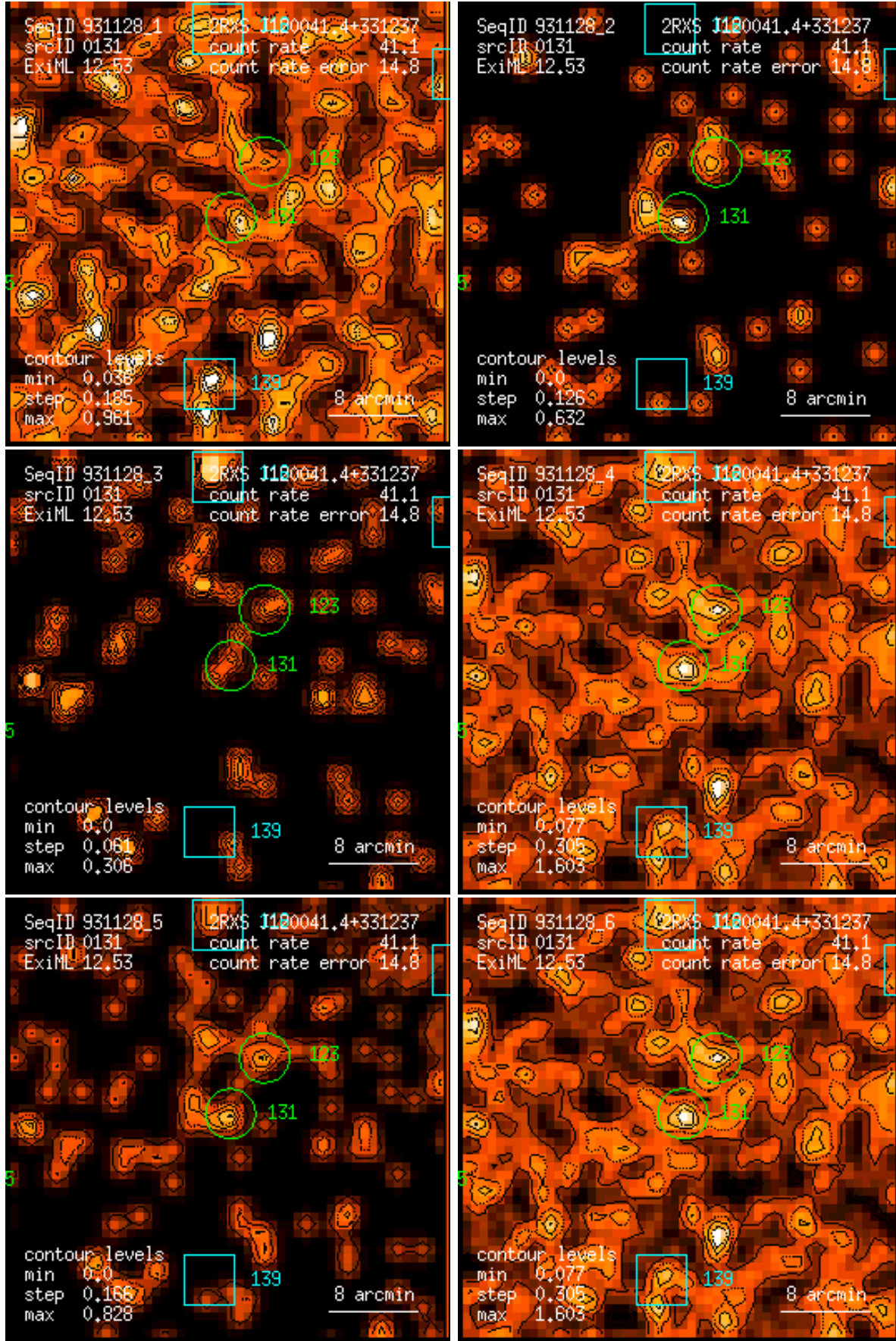
Figure 131: RASS 931128: detection 0131: band rate images, Gaussian filter: (1) PSPC channels 11 – 41, (2) 52 – 90, (3) 91 – 201, (4) 11 – 235, (5) 52 – 201, (6) 11 – 201. Broad band rates in counts/ks. Band rate contour levels in counts/ks/arcmin 2 .
