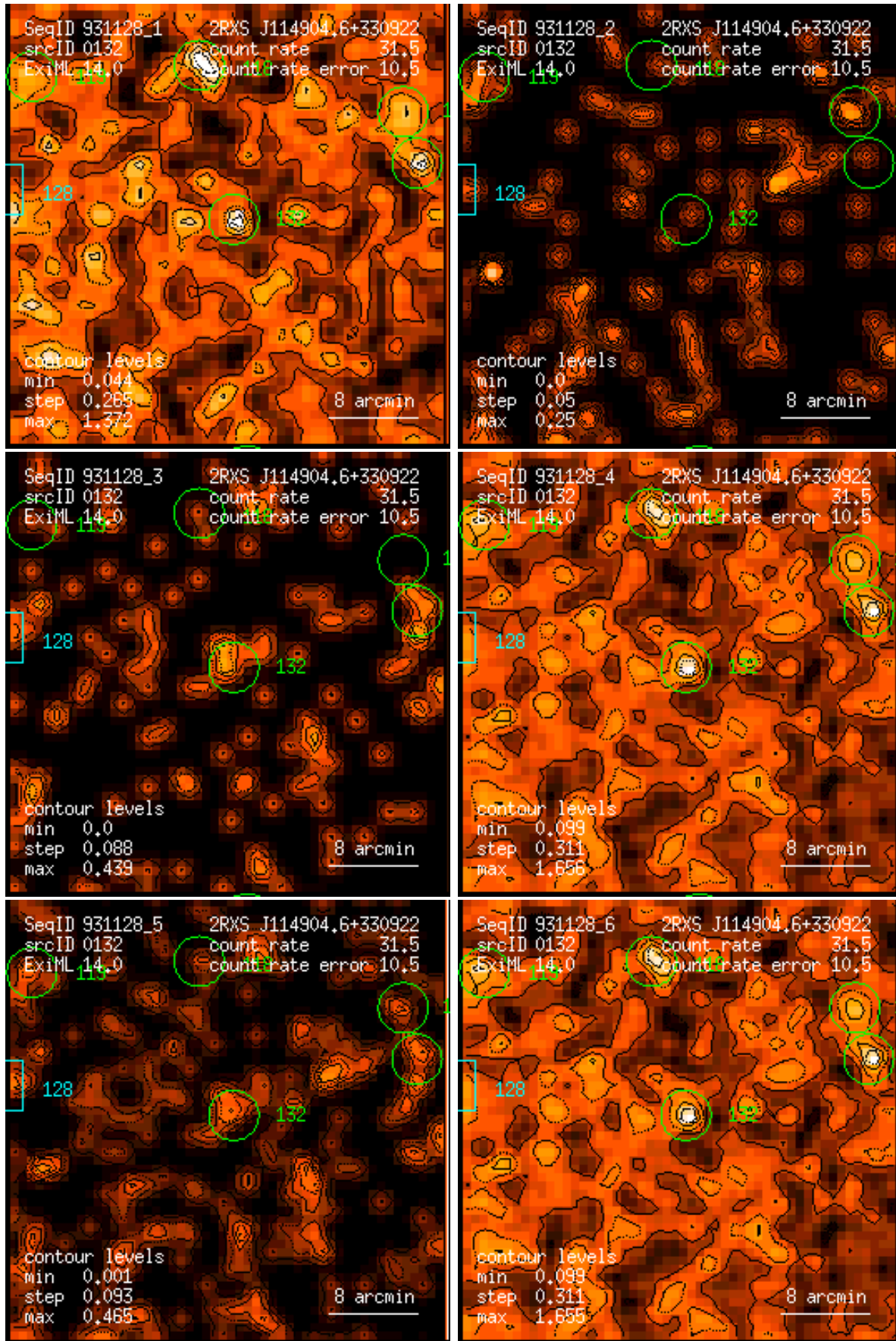
Figure 132: RASS 931128: detection 0132: band rate images, Gaussian filter: (1) PSPC channels 11 – 41, (2) 52 – 90, (3) 91 – 201, (4) 11 – 235, (5) 52 – 201, (6) 11 – 201. Broad band rates in counts/ks. Band rate contour levels in counts/ks/arcmin 2 .
