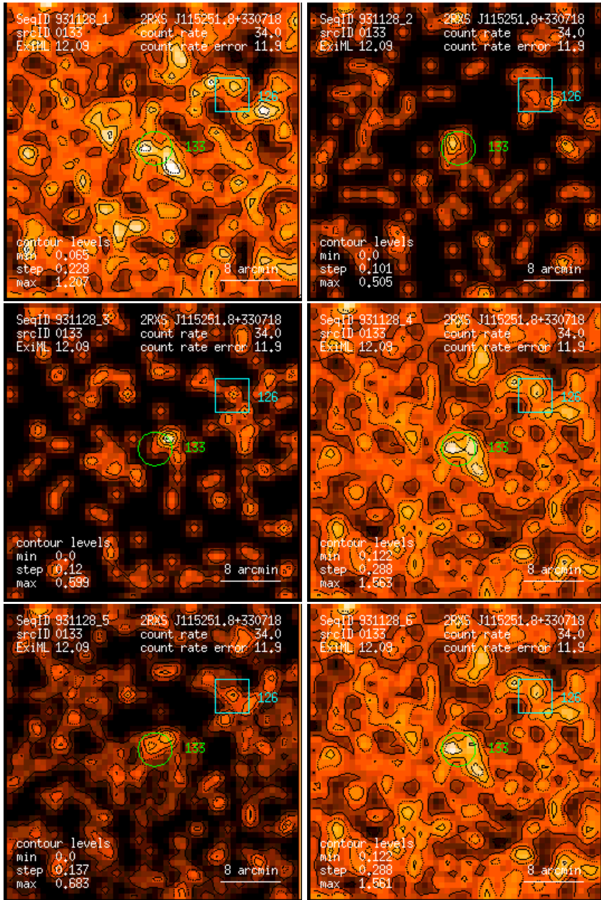
Figure 133: RASS 931128: detection 0133: band rate images, Gaussian filter: (1) PSPC channels 11 – 41, (2) 52 – 90, (3) 91 – 201, (4) 11 – 235, (5) 52 – 201, (6) 11 – 201. Broad band rates in counts/ks. Band rate contour levels in counts/ks/arcmin 2 .
