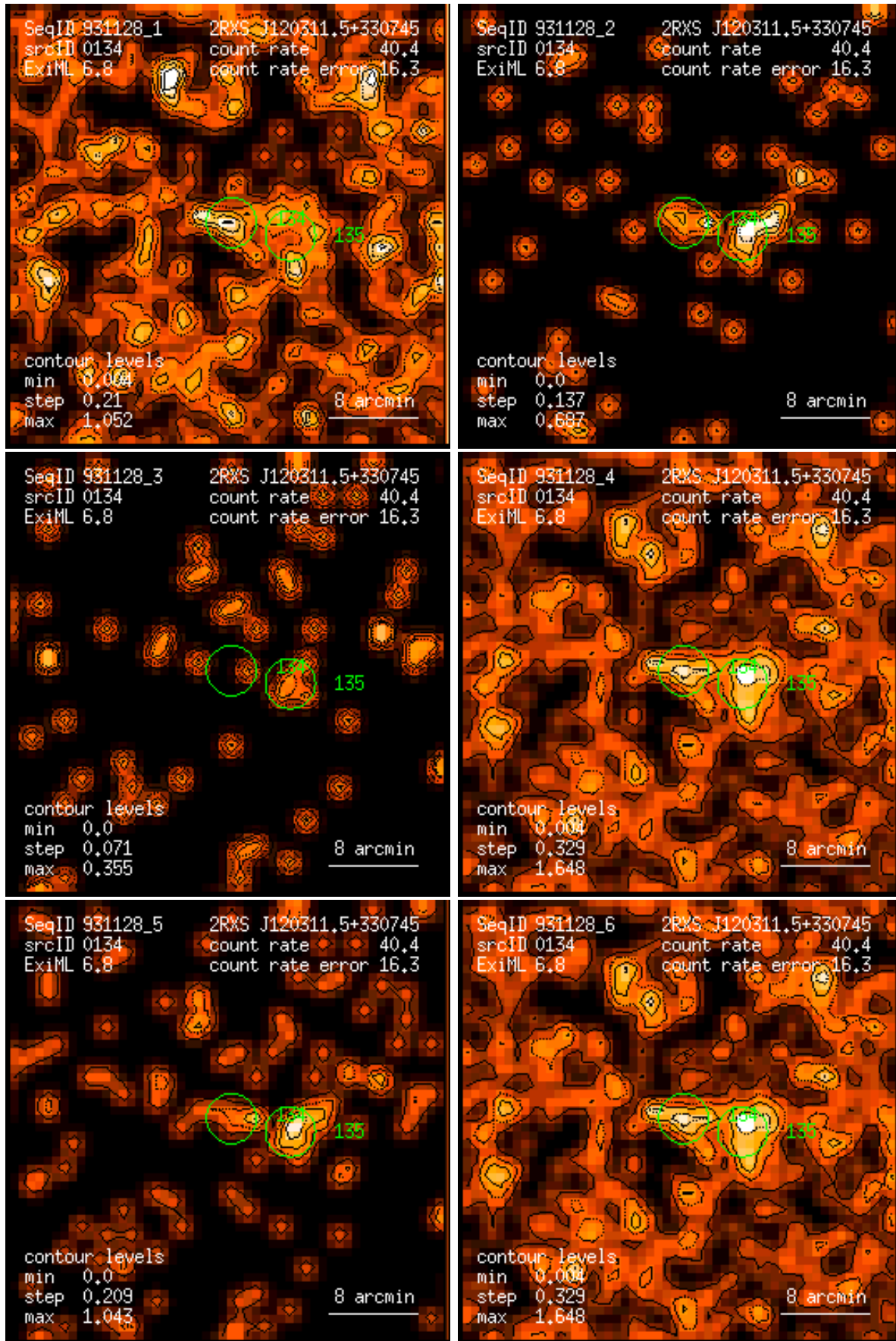
Figure 134: RASS 931128: detection 0134: band rate images, Gaussian filter: (1) PSPC channels 11 – 41, (2) 52 – 90, (3) 91 – 201, (4) 11 – 235, (5) 52 – 201, (6) 11 – 201. Broad band rates in counts/ks. Band rate contour levels in counts/ks/arcmin 2 .
