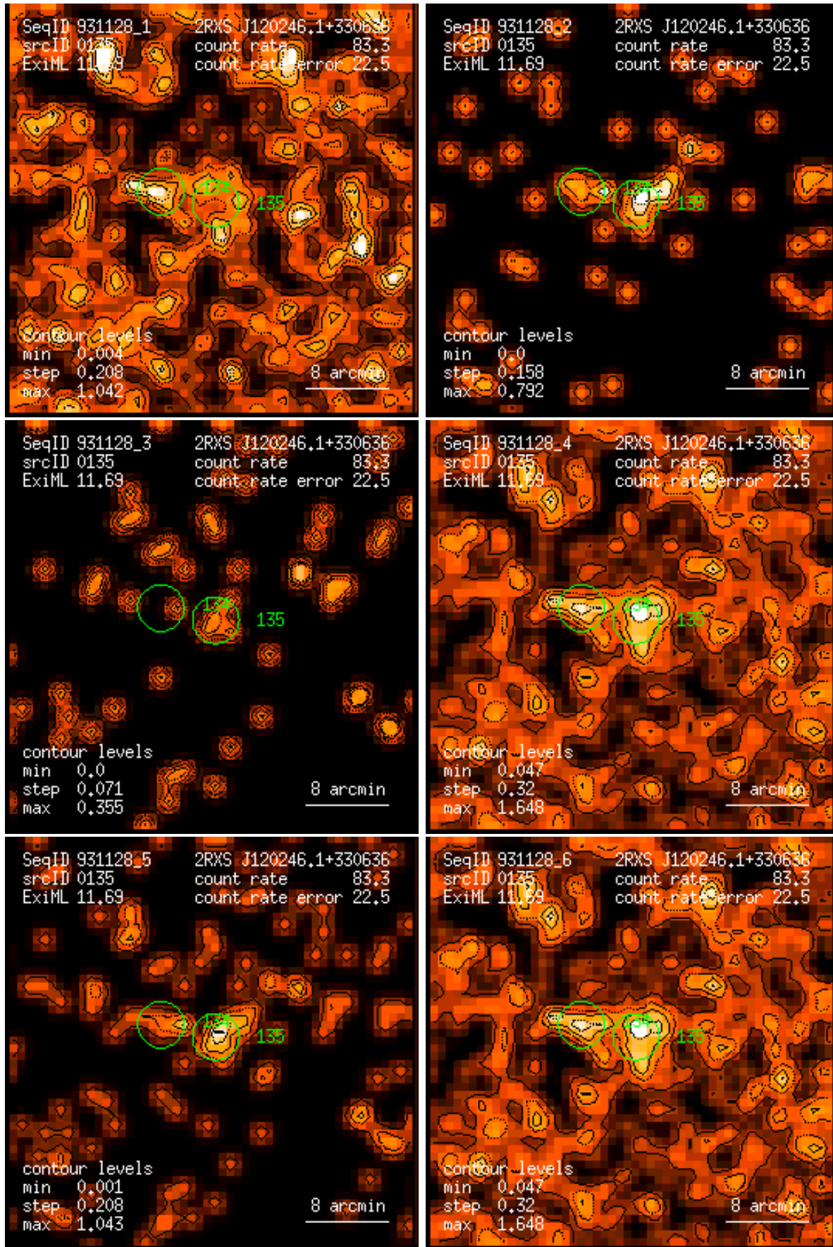
Figure 135: RASS 931128: detection 0135: band rate images, Gaussian filter: (1) PSPC channels 11 – 41, (2) 52 – 90, (3) 91 – 201, (4) 11 – 235, (5) 52 – 201, (6) 11 – 201. Broad band rates in counts/ks. Band rate contour levels in counts/ks/arcmin 2 .
