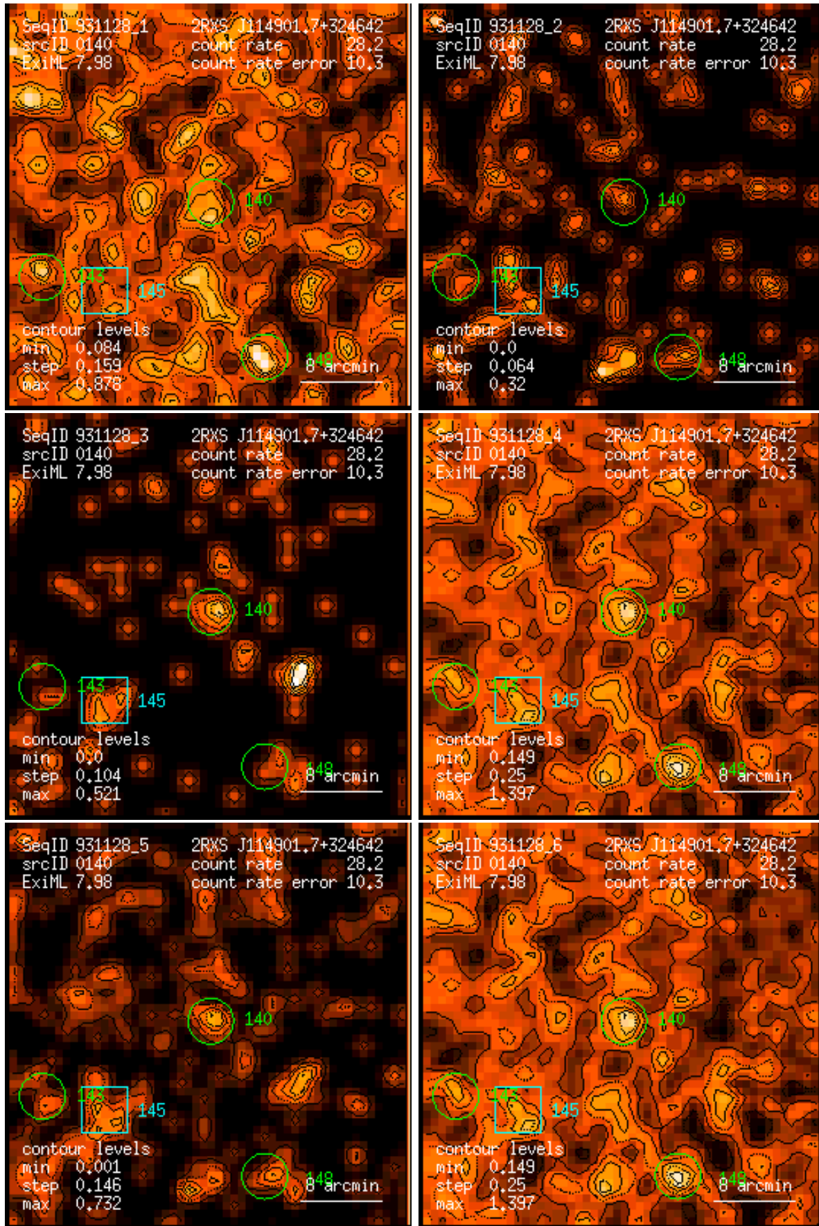
Figure 140: RASS 931128: detection 0140: band rate images, Gaussian filter: (1) PSPC channels 11 – 41, (2) 52 – 90, (3) 91 – 201, (4) 11 – 235, (5) 52 – 201, (6) 11 – 201. Broad band rates in counts/ks. Band rate contour levels in counts/ks/arcmin 2 .
