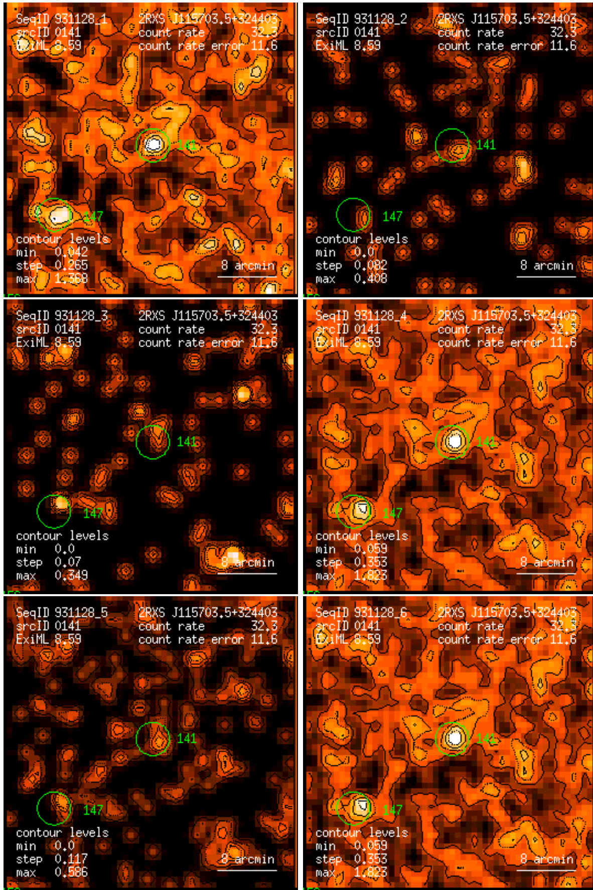
Figure 141: RASS 931128: detection 0141: band rate images, Gaussian filter: (1) PSPC channels 11 – 41, (2) 52 – 90, (3) 91 – 201, (4) 11 – 235, (5) 52 – 201, (6) 11 – 201. Broad band rates in counts/ks. Band rate contour levels in counts/ks/arcmin 2 .
