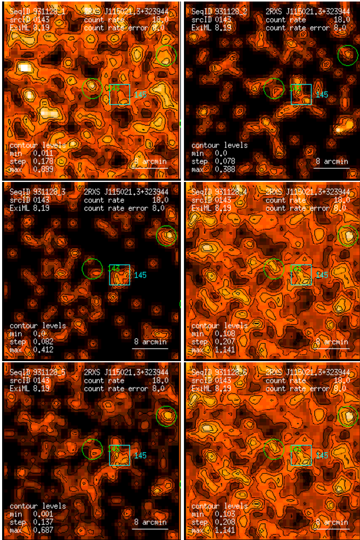
Figure 143: RASS 931128: detection 0143: band rate images, Gaussian filter: (1) PSPC channels 11 – 41, (2) 52 – 90, (3) 91 – 201, (4) 11 – 235, (5) 52 – 201, (6) 11 – 201. Broad band rates in counts/ks. Band rate contour levels in counts/ks/arcmin 2 .
