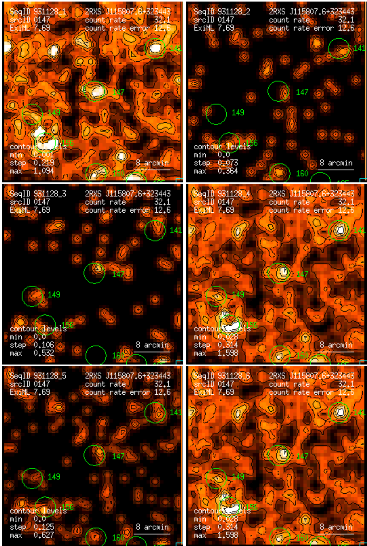
Figure 147: RASS 931128: detection 0147: band rate images, Gaussian filter: (1) PSPC channels 11 – 41, (2) 52 – 90, (3) 91 – 201, (4) 11 – 235, (5) 52 – 201, (6) 11 – 201. Broad band rates in counts/ks. Band rate contour levels in counts/ks/arcmin 2 .
