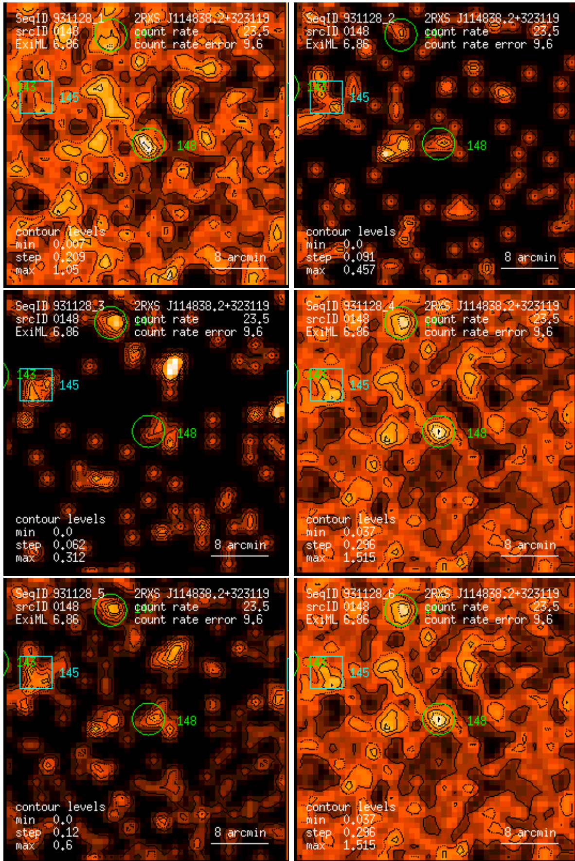
Figure 148: RASS 931128: detection 0148: band rate images, Gaussian filter: (1) PSPC channels 11 – 41, (2) 52 – 90, (3) 91 – 201, (4) 11 – 235, (5) 52 – 201, (6) 11 – 201. Broad band rates in counts/ks. Band rate contour levels in counts/ks/arcmin 2 .
