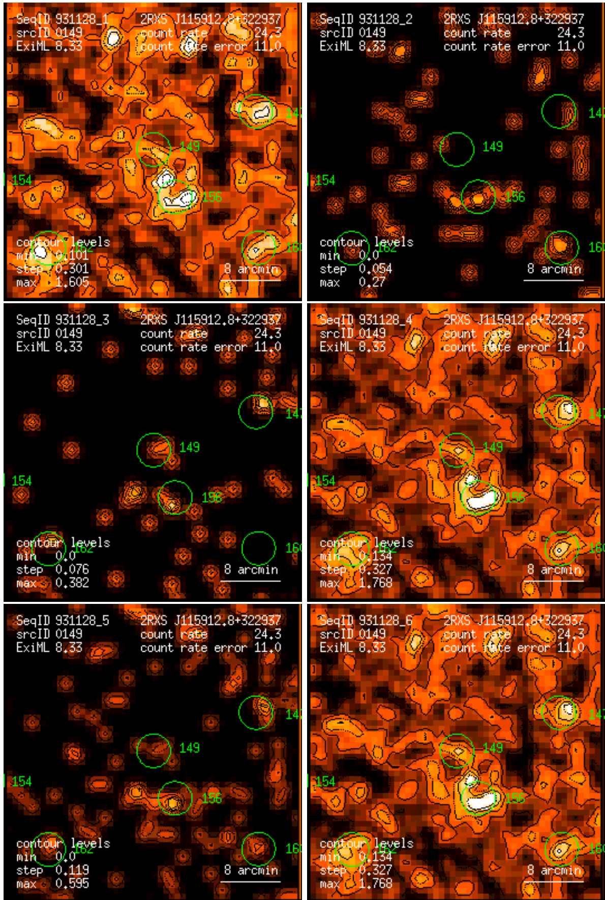
Figure 149: RASS 931128: detection 0149: band rate images, Gaussian filter: (1) PSPC channels 11 – 41, (2) 52 – 90, (3) 91 – 201, (4) 11 – 235, (5) 52 – 201, (6) 11 – 201. Broad band rates in counts/ks. Band rate contour levels in counts/ks/arcmin 2 .
