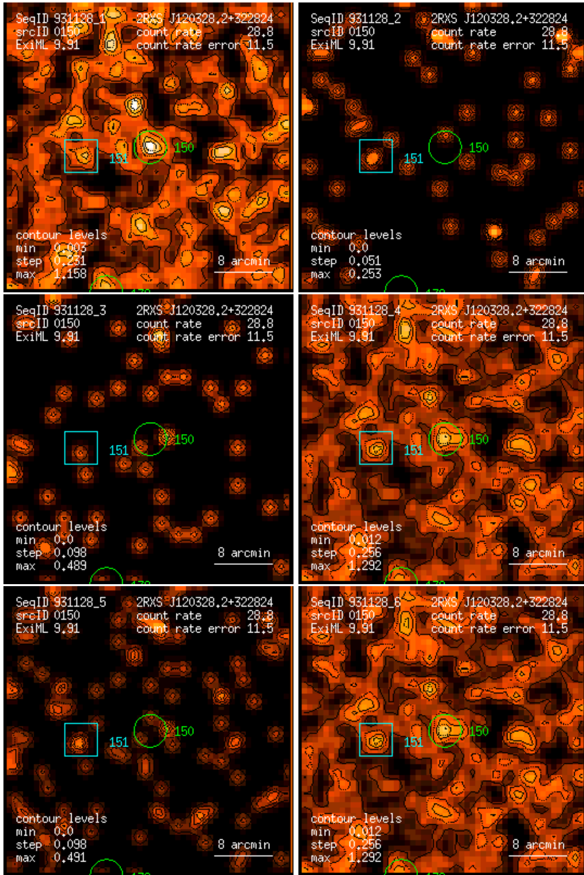
Figure 150: RASS 931128: detection 0150: band rate images, Gaussian filter: (1) PSPC channels 11 – 41, (2) 52 – 90, (3) 91 – 201, (4) 11 – 235, (5) 52 – 201, (6) 11 – 201. Broad band rates in counts/ks. Band rate contour levels in counts/ks/arcmin 2 .
