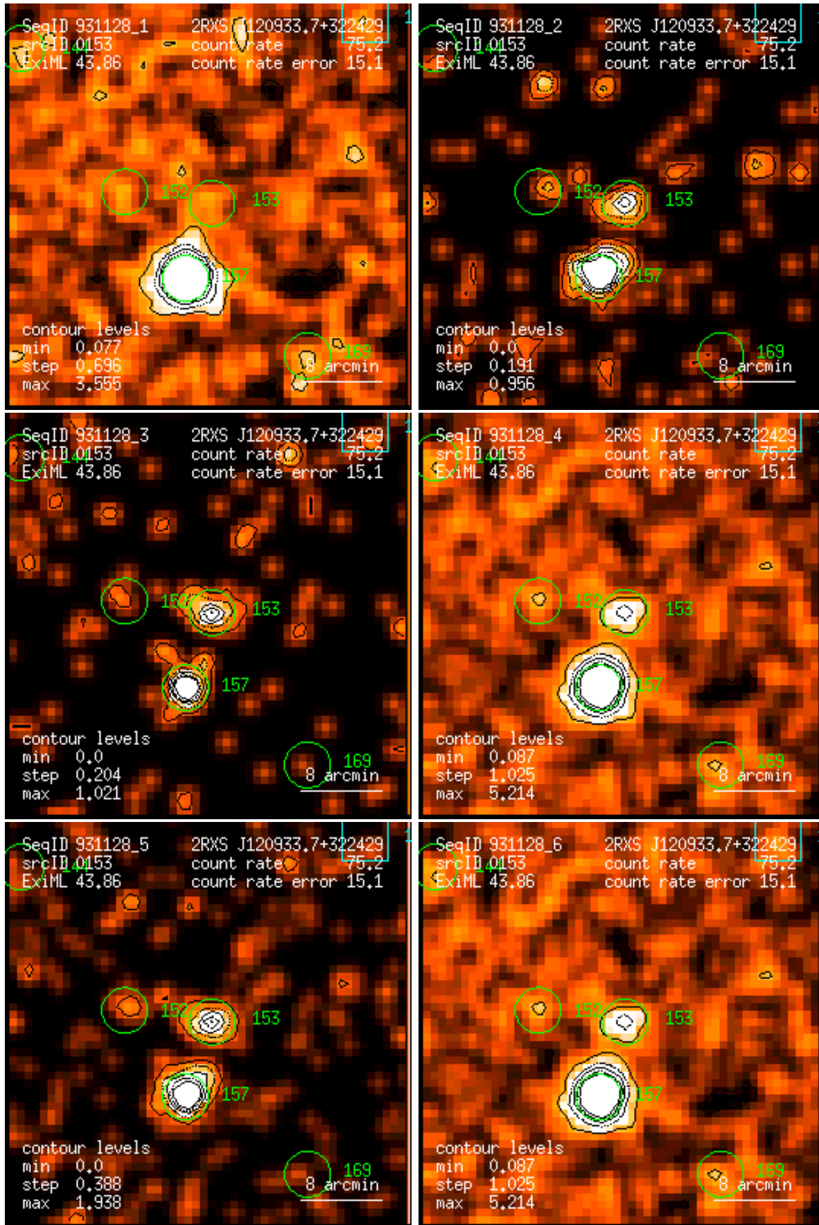
Figure 153: RASS 931128: detection 0153: band rate images, Gaussian filter: (1) PSPC channels 11 – 41, (2) 52 – 90, (3) 91 – 201, (4) 11 – 235, (5) 52 – 201, (6) 11 – 201. Broad band rates in counts/ks. Band rate contour levels in counts/ks/arcmin 2 .
