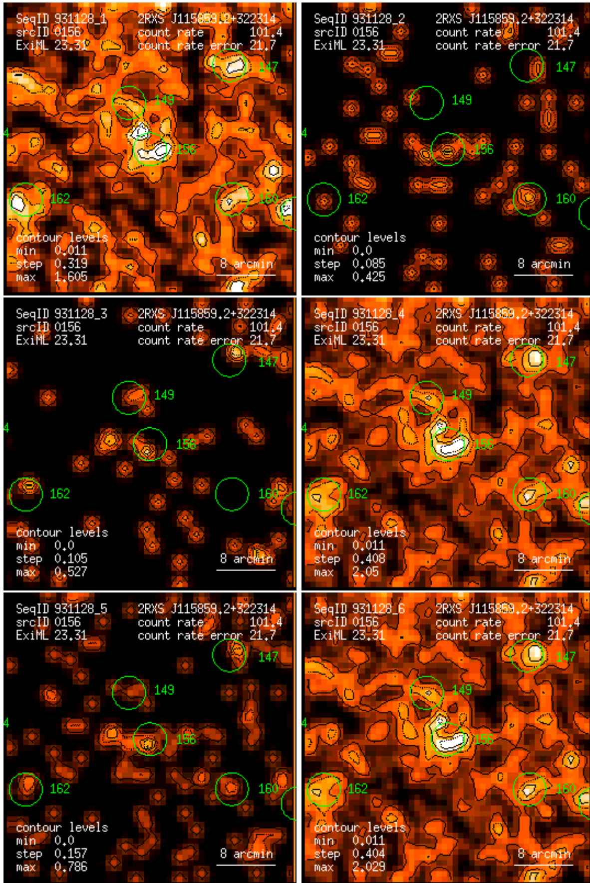
Figure 156: RASS 931128: detection 0156: band rate images, Gaussian filter: (1) PSPC channels 11 – 41, (2) 52 – 90, (3) 91 – 201, (4) 11 – 235, (5) 52 – 201, (6) 11 – 201. Broad band rates in counts/ks. Band rate contour levels in counts/ks/arcmin 2 .
