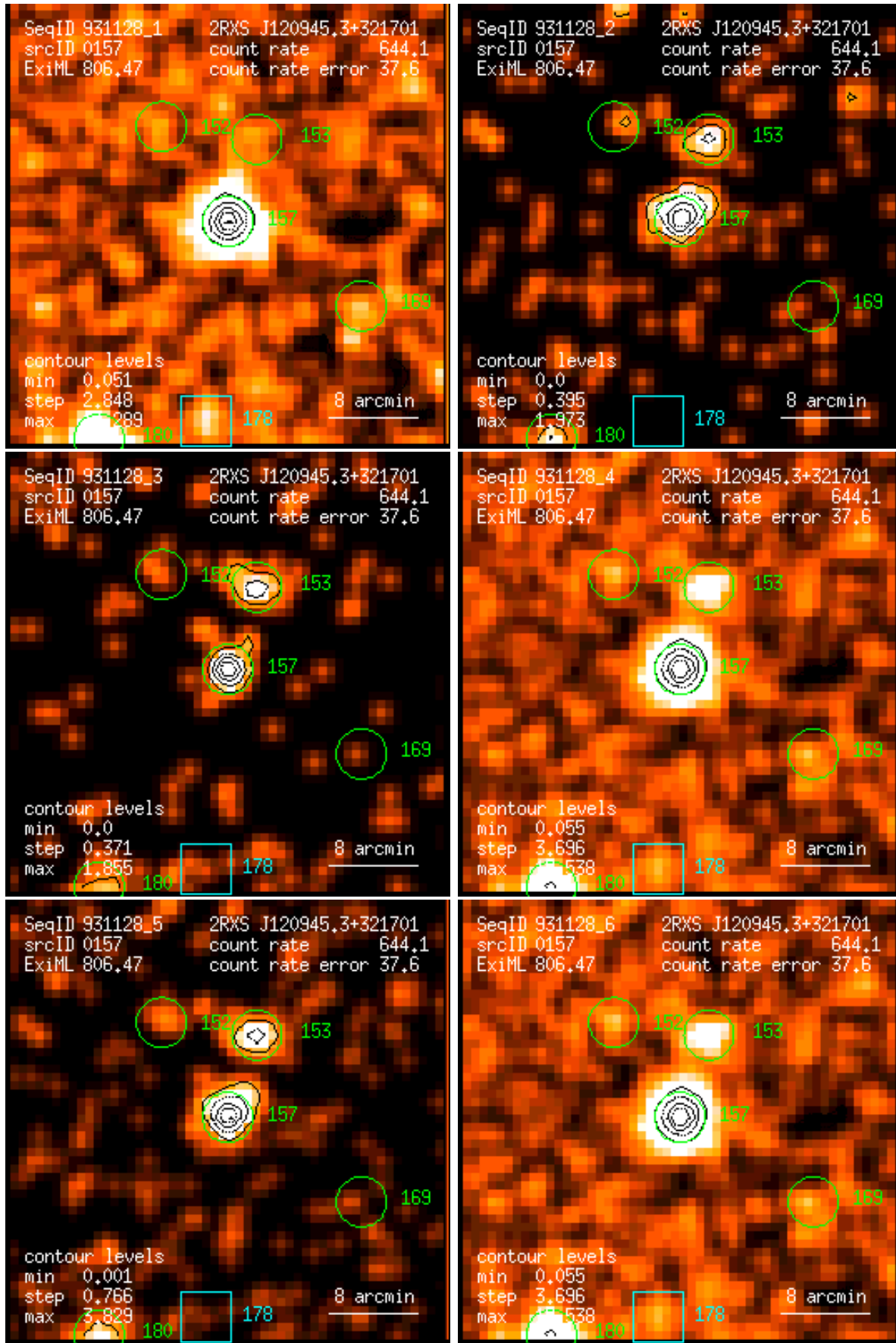
Figure 157: RASS 931128: detection 0157: band rate images, Gaussian filter: (1) PSPC channels 11 – 41, (2) 52 – 90, (3) 91 – 201, (4) 11 – 235, (5) 52 – 201, (6) 11 – 201. Broad band rates in counts/ks. Band rate contour levels in counts/ks/arcmin 2 .
