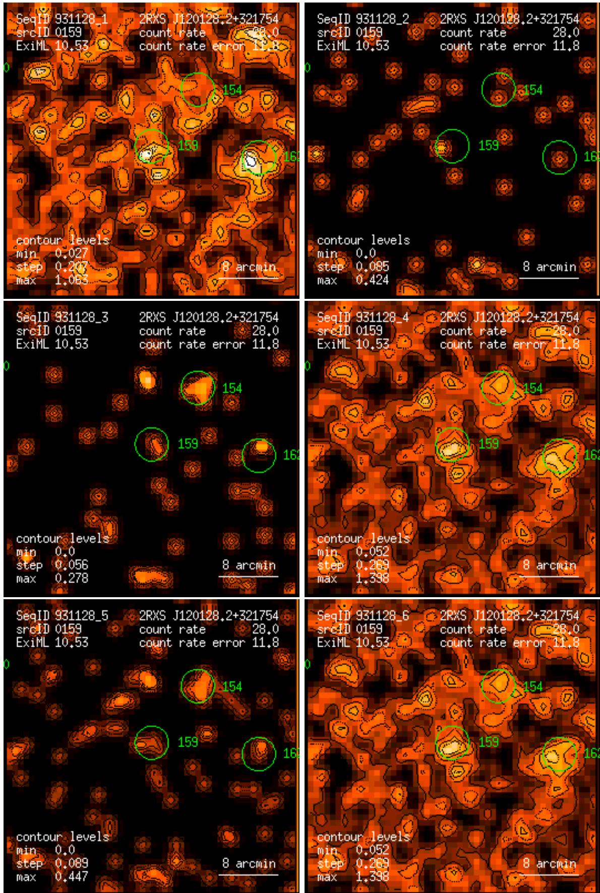
Figure 159: RASS 931128: detection 0159: band rate images, Gaussian filter: (1) PSPC channels 11 – 41, (2) 52 – 90, (3) 91 – 201, (4) 11 – 235, (5) 52 – 201, (6) 11 – 201. Broad band rates in counts/ks. Band rate contour levels in counts/ks/arcmin 2 .
