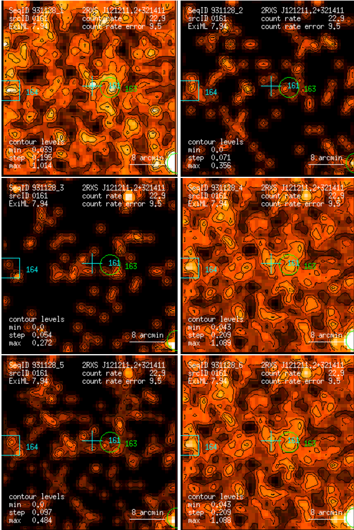
Figure 161: RASS 931128: detection 0161: band rate images, Gaussian filter: (1) PSPC channels 11 – 41, (2) 52 – 90, (3) 91 – 201, (4) 11 – 235, (5) 52 – 201, (6) 11 – 201. Broad band rates in counts/ks. Band rate contour levels in counts/ks/arcmin 2 .
