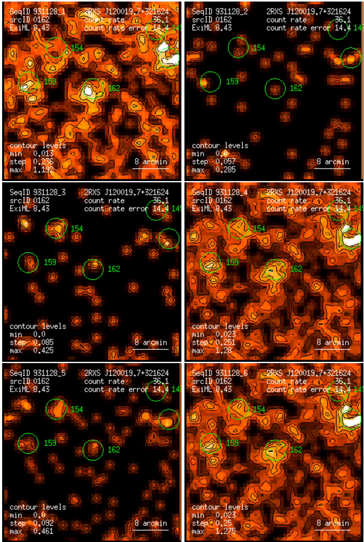
Figure 162: RASS 931128: detection 0162: band rate images, Gaussian filter: (1) PSPC channels 11 – 41, (2) 52 – 90, (3) 91 – 201, (4) 11 – 235, (5) 52 – 201, (6) 11 – 201. Broad band rates in counts/ks. Band rate contour levels in counts/ks/arcmin 2 .
