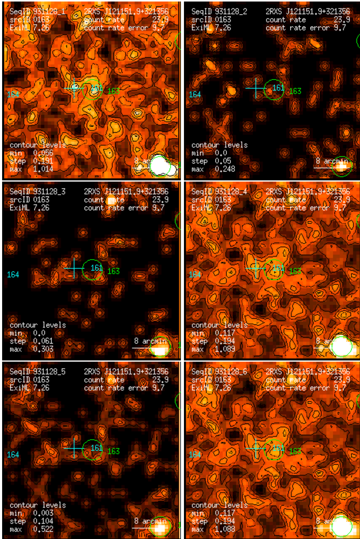
Figure 163: RASS 931128: detection 0163: band rate images, Gaussian filter: (1) PSPC channels 11 – 41, (2) 52 – 90, (3) 91 – 201, (4) 11 – 235, (5) 52 – 201, (6) 11 – 201. Broad band rates in counts/ks. Band rate contour levels in counts/ks/arcmin 2 .
