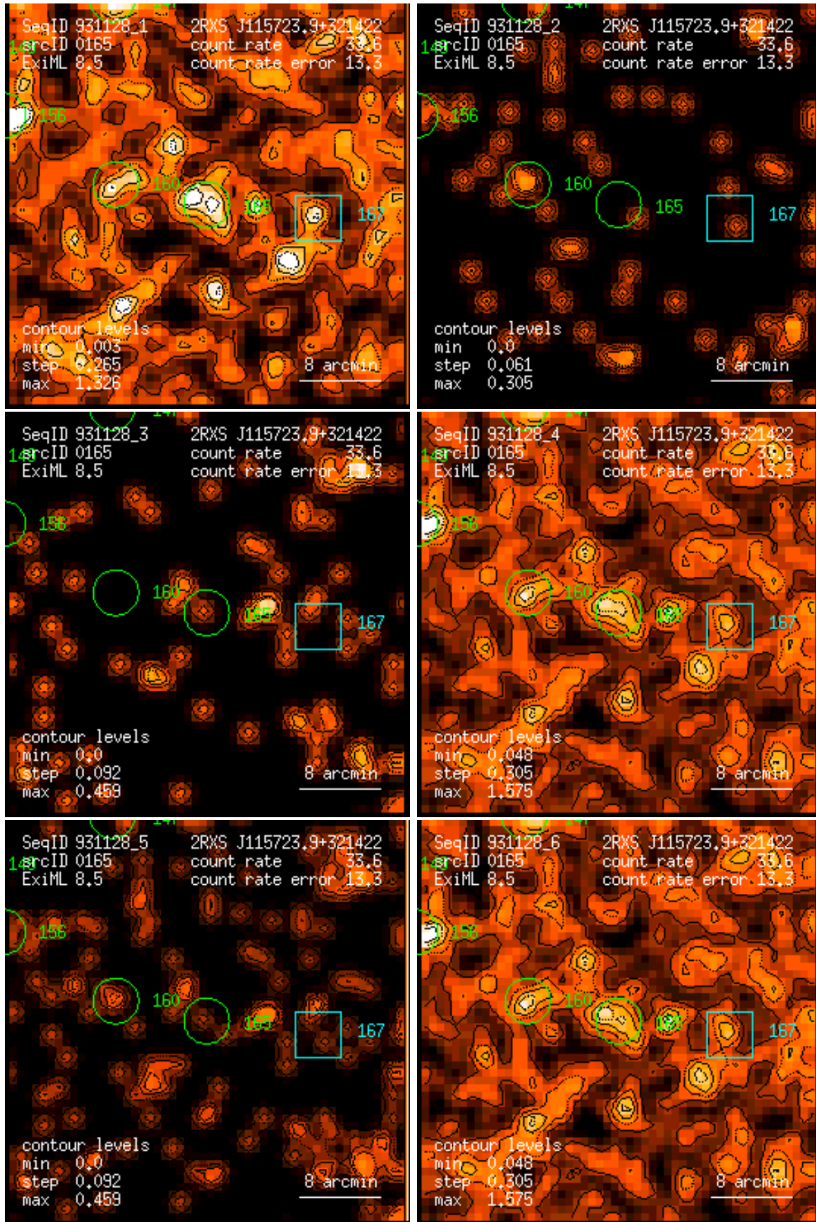
Figure 165: RASS 931128: detection 0165: band rate images, Gaussian filter: (1) PSPC channels 11 – 41, (2) 52 – 90, (3) 91 – 201, (4) 11 – 235, (5) 52 – 201, (6) 11 – 201. Broad band rates in counts/ks. Band rate contour levels in counts/ks/arcmin 2 .
