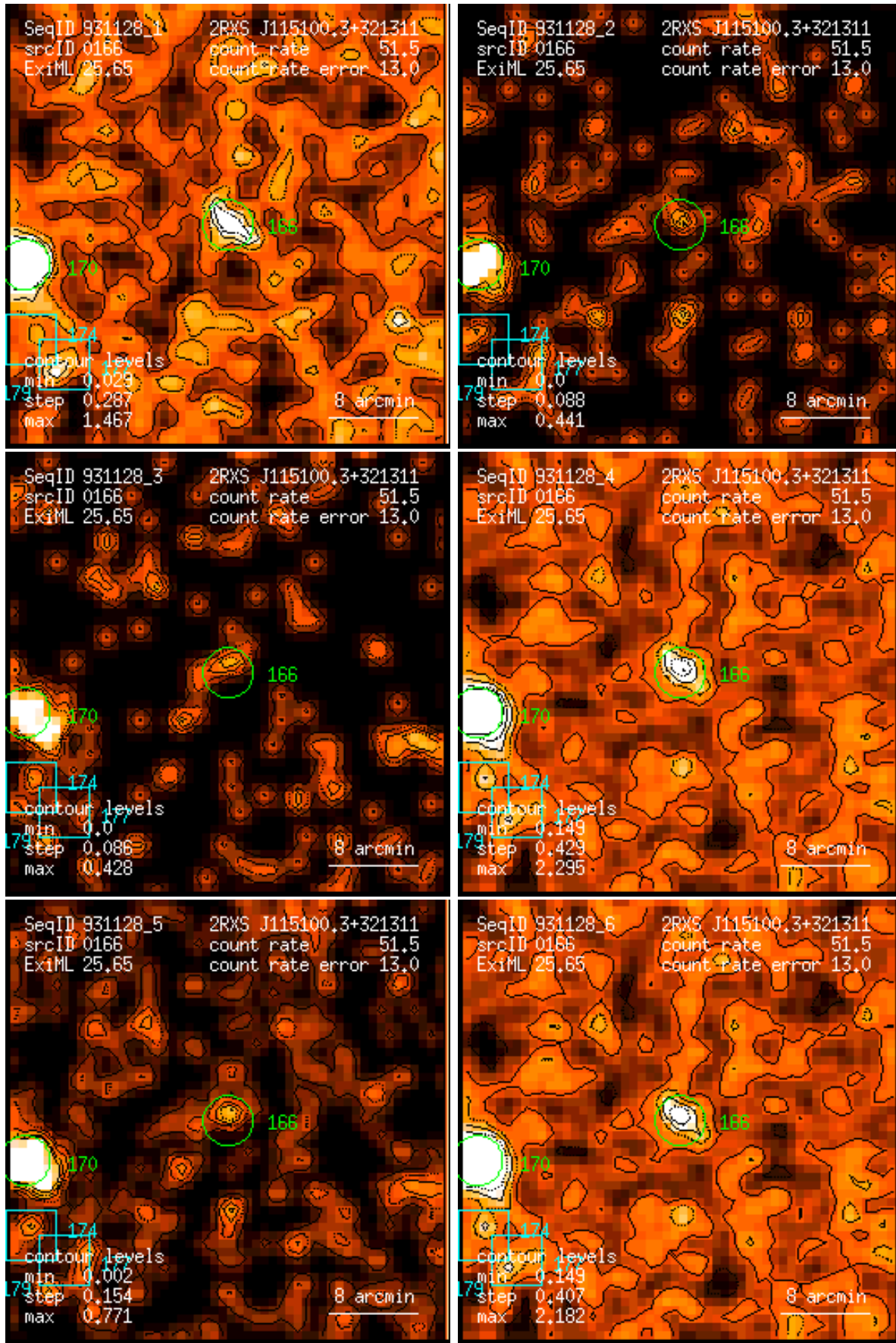
Figure 166: RASS 931128: detection 0166: band rate images, Gaussian filter: (1) PSPC channels 11 – 41, (2) 52 – 90, (3) 91 – 201, (4) 11 – 235, (5) 52 – 201, (6) 11 – 201. Broad band rates in counts/ks. Band rate contour levels in counts/ks/arcmin 2 .
