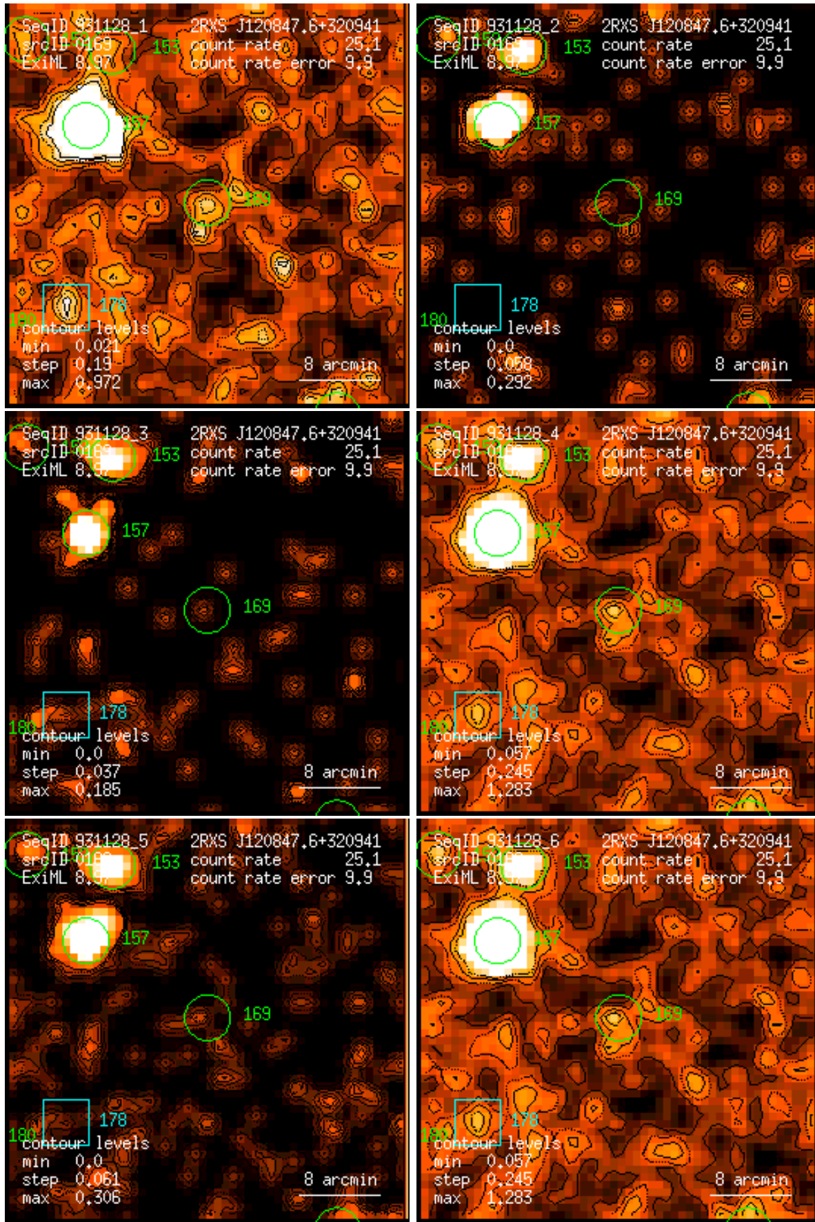
Figure 169: RASS 931128: detection 0169: band rate images, Gaussian filter: (1) PSPC channels 11 – 41, (2) 52 – 90, (3) 91 – 201, (4) 11 – 235, (5) 52 – 201, (6) 11 – 201. Broad band rates in counts/ks. Band rate contour levels in counts/ks/arcmin 2 .
