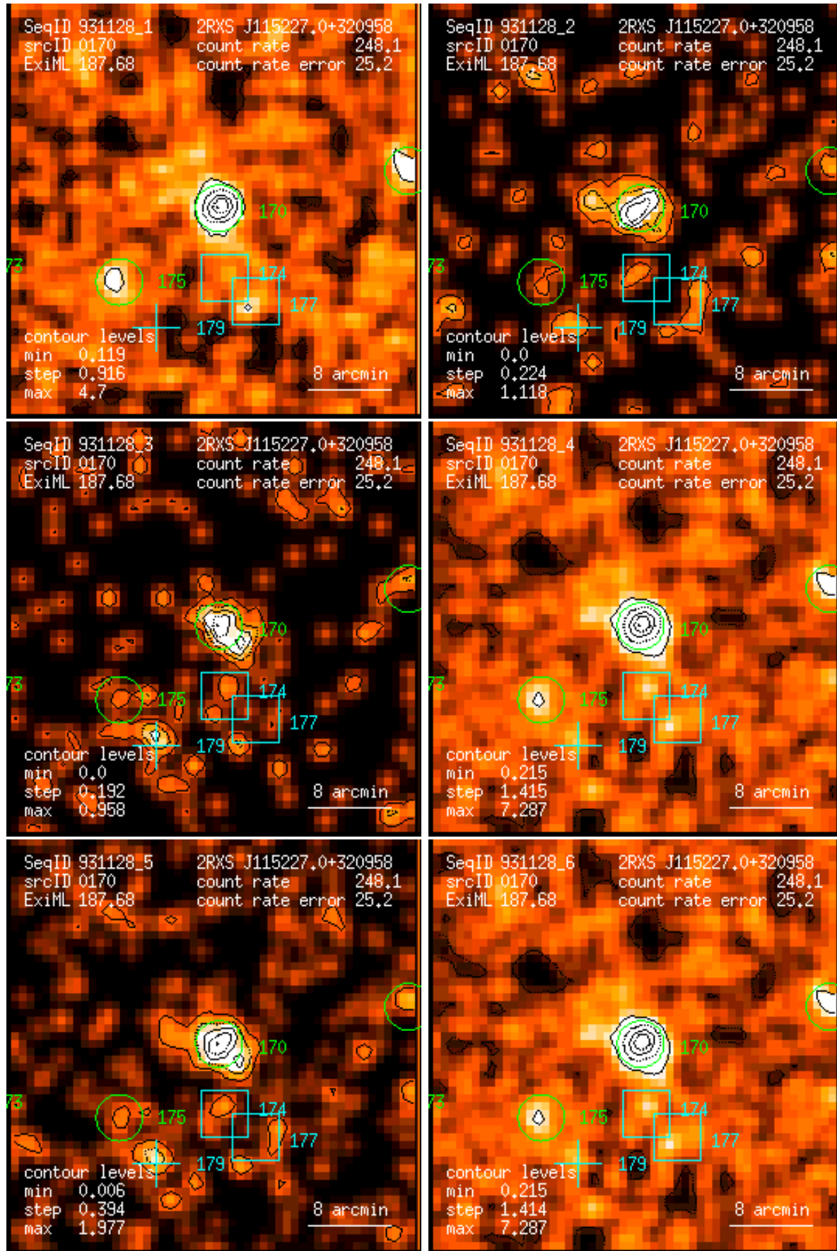
Figure 170: RASS 931128: detection 0170: band rate images, Gaussian filter: (1) PSPC channels 11 – 41, (2) 52 – 90, (3) 91 – 201, (4) 11 – 235, (5) 52 – 201, (6) 11 – 201. Broad band rates in counts/ks. Band rate contour levels in counts/ks/arcmin 2 .
