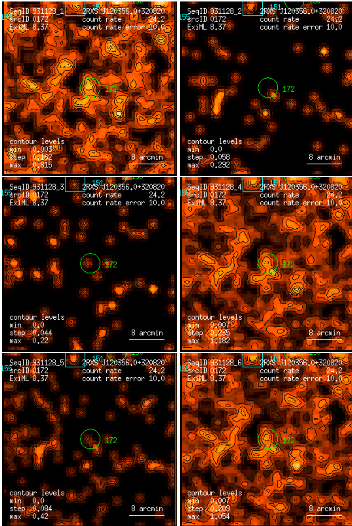
Figure 172: RASS 931128: detection 0172: band rate images, Gaussian filter: (1) PSPC channels 11 – 41, (2) 52 – 90, (3) 91 – 201, (4) 11 – 235, (5) 52 – 201, (6) 11 – 201. Broad band rates in counts/ks. Band rate contour levels in counts/ks/arcmin 2 .
