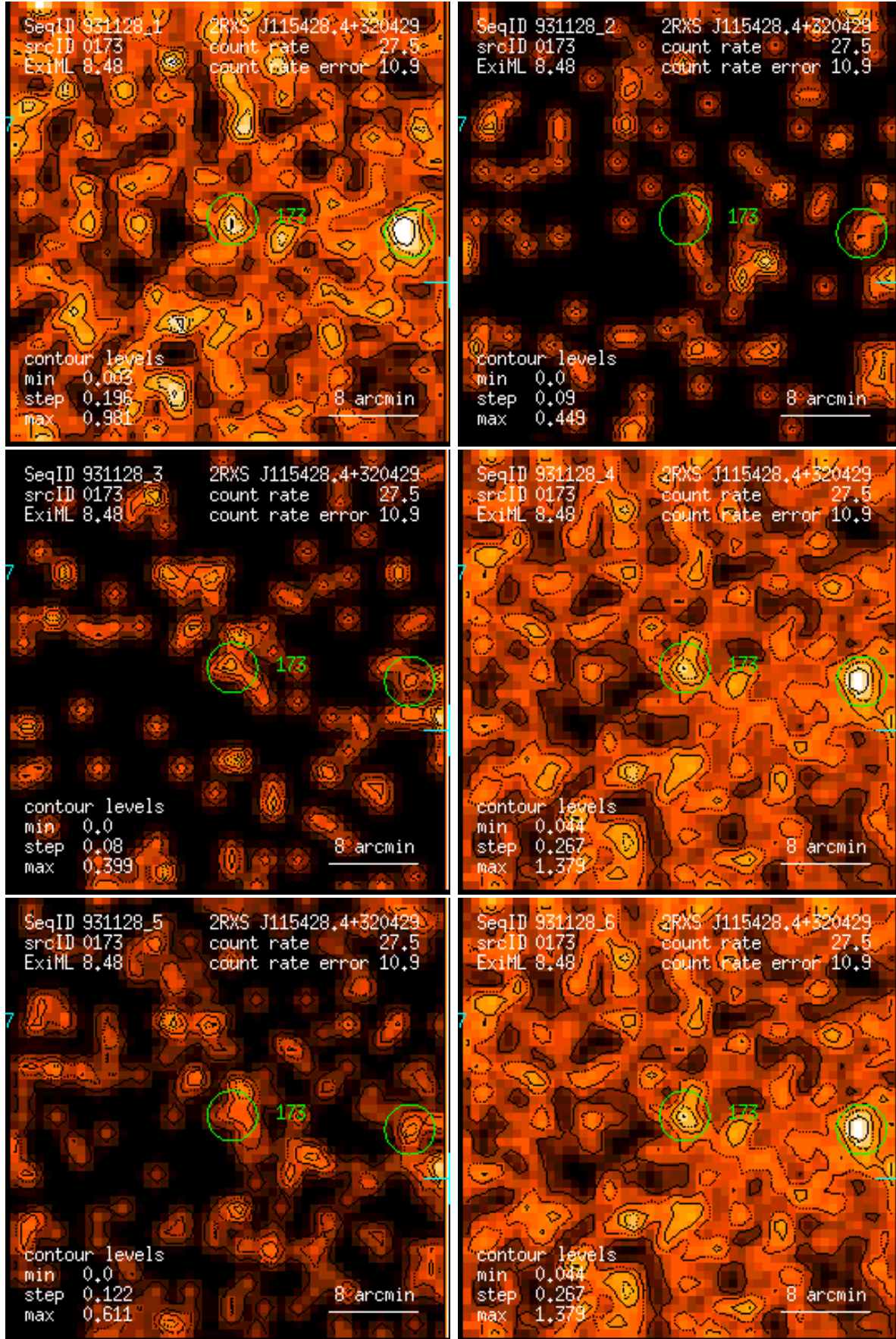
Figure 173: RASS 931128: detection 0173: band rate images, Gaussian filter: (1) PSPC channels 11 – 41, (2) 52 – 90, (3) 91 – 201, (4) 11 – 235, (5) 52 – 201, (6) 11 – 201. Broad band rates in counts/ks. Band rate contour levels in counts/ks/arcmin 2 .
