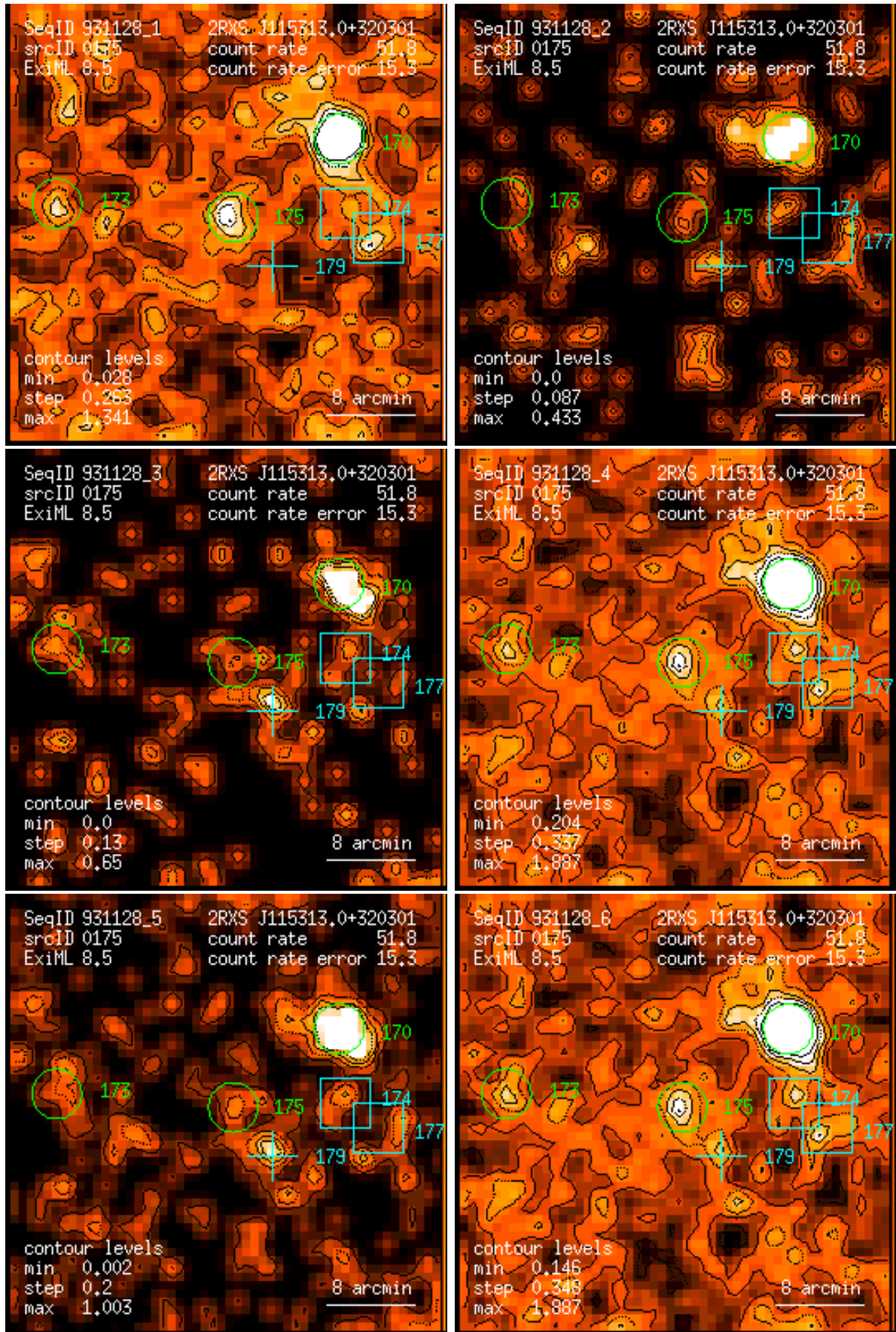
Figure 175: RASS 931128: detection 0175: band rate images, Gaussian filter: (1) PSPC channels 11 – 41, (2) 52 – 90, (3) 91 – 201, (4) 11 – 235, (5) 52 – 201, (6) 11 – 201. Broad band rates in counts/ks. Band rate contour levels in counts/ks/arcmin 2 .
