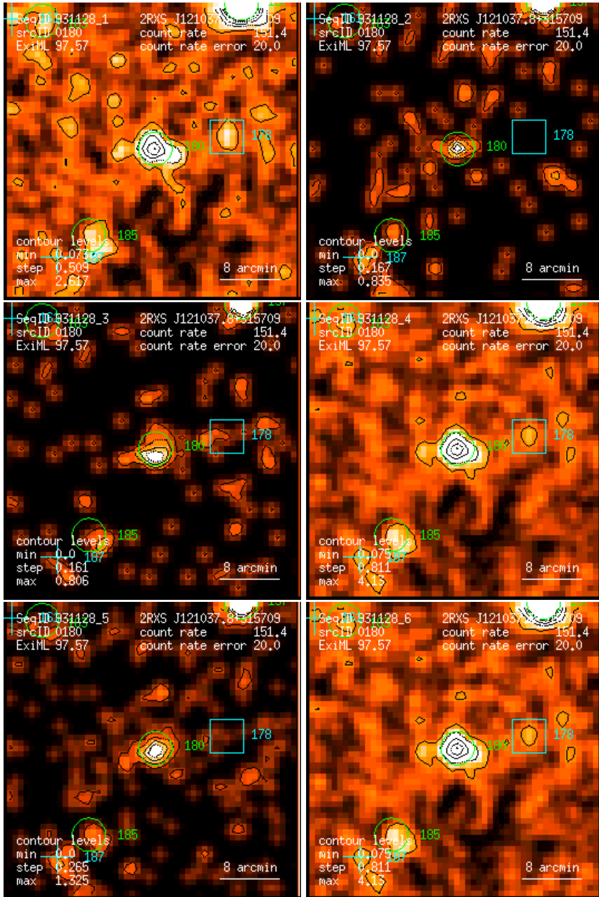
Figure 180: RASS 931128: detection 0180: band rate images, Gaussian filter: (1) PSPC channels 11 – 41, (2) 52 – 90, (3) 91 – 201, (4) 11 – 235, (5) 52 – 201, (6) 11 – 201. Broad band rates in counts/ks. Band rate contour levels in counts/ks/arcmin 2 .
