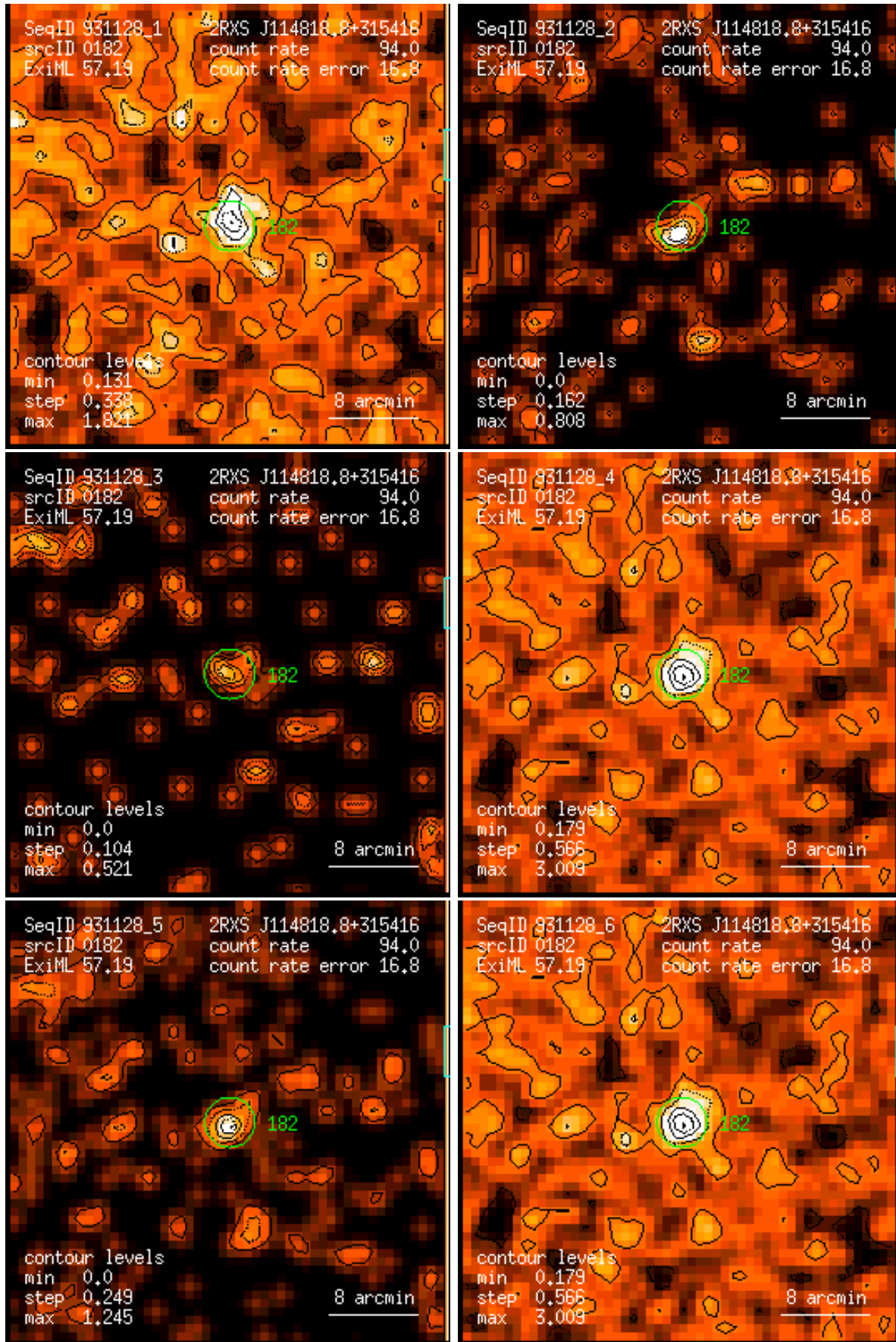
Figure 182: RASS 931128: detection 0182: band rate images, Gaussian filter: (1) PSPC channels 11 – 41, (2) 52 – 90, (3) 91 – 201, (4) 11 – 235, (5) 52 – 201, (6) 11 – 201. Broad band rates in counts/ks. Band rate contour levels in counts/ks/arcmin 2 .
