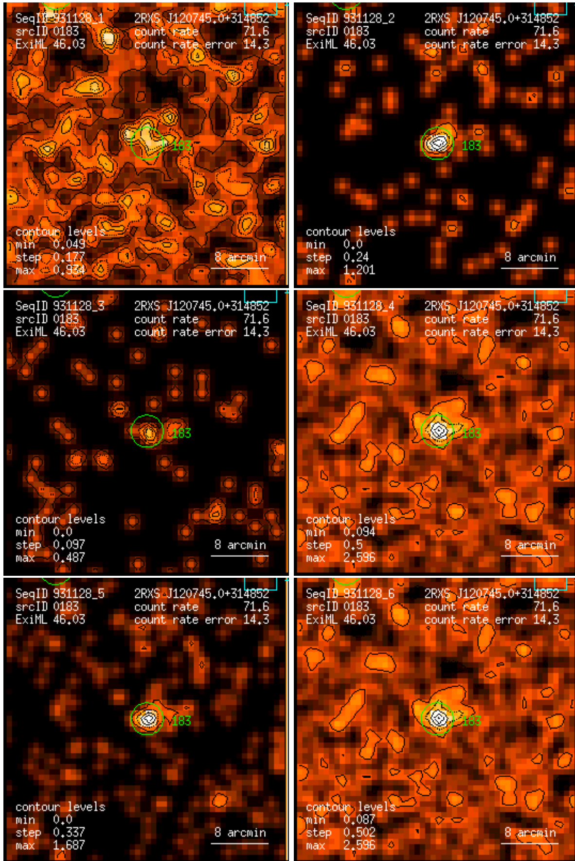
Figure 183: RASS 931128: detection 0183: band rate images, Gaussian filter: (1) PSPC channels 11 – 41, (2) 52 – 90, (3) 91 – 201, (4) 11 – 235, (5) 52 – 201, (6) 11 – 201. Broad band rates in counts/ks. Band rate contour levels in counts/ks/arcmin 2 .
