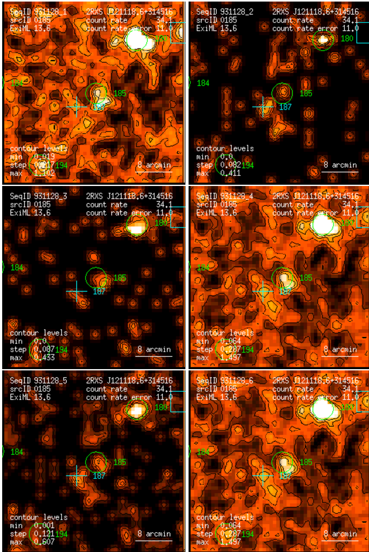
Figure 185: RASS 931128: detection 0185: band rate images, Gaussian filter: (1) PSPC channels 11 – 41, (2) 52 – 90, (3) 91 – 201, (4) 11 – 235, (5) 52 – 201, (6) 11 – 201. Broad band rates in counts/ks. Band rate contour levels in counts/ks/arcmin 2 .
