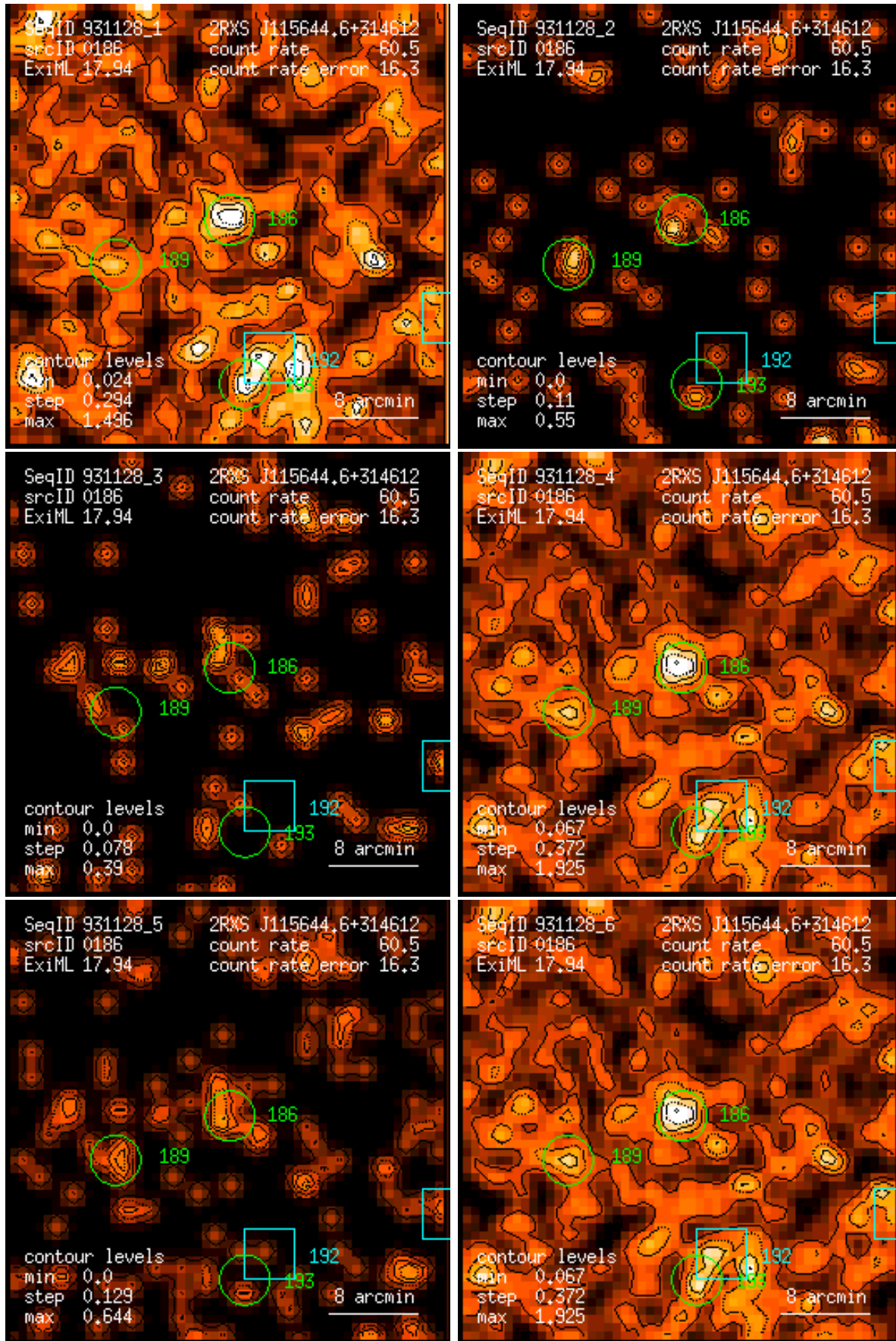
Figure 186: RASS 931128: detection 0186: band rate images, Gaussian filter: (1) PSPC channels 11 – 41, (2) 52 – 90, (3) 91 – 201, (4) 11 – 235, (5) 52 – 201, (6) 11 – 201. Broad band rates in counts/ks. Band rate contour levels in counts/ks/arcmin 2 .
