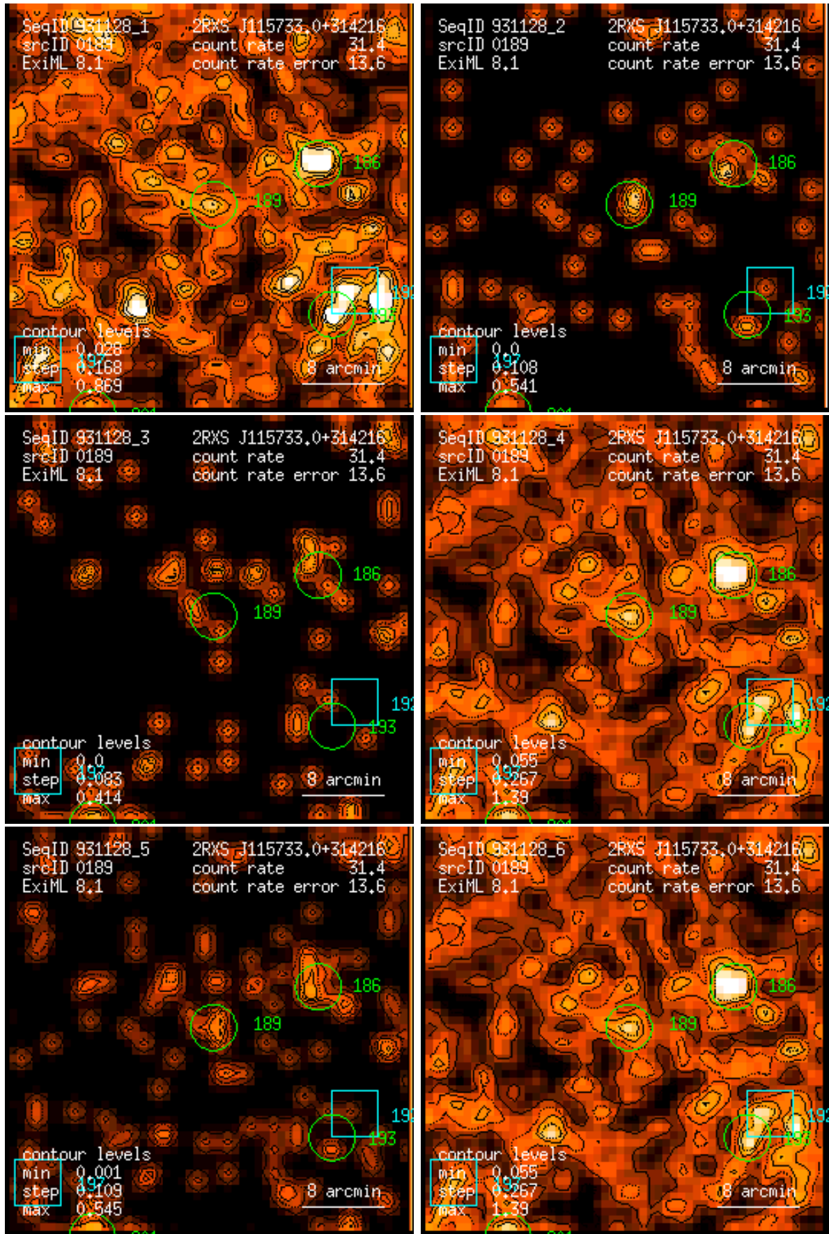
Figure 189: RASS 931128: detection 0189: band rate images, Gaussian filter: (1) PSPC channels 11 – 41, (2) 52 – 90, (3) 91 – 201, (4) 11 – 235, (5) 52 – 201, (6) 11 – 201. Broad band rates in counts/ks. Band rate contour levels in counts/ks/arcmin 2 .
